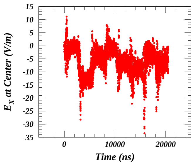
ECLOUD-TS0608_SEY20_Epk310: Electric Field at Beam
