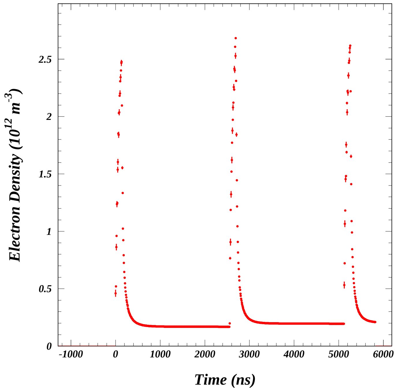
Job 35720: Beampipe-averaged Cloud Density ( 10^{12} \text{ m}^{-3} )
