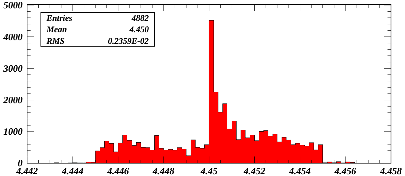
Charge-weighted \rho Distribution (cm)
