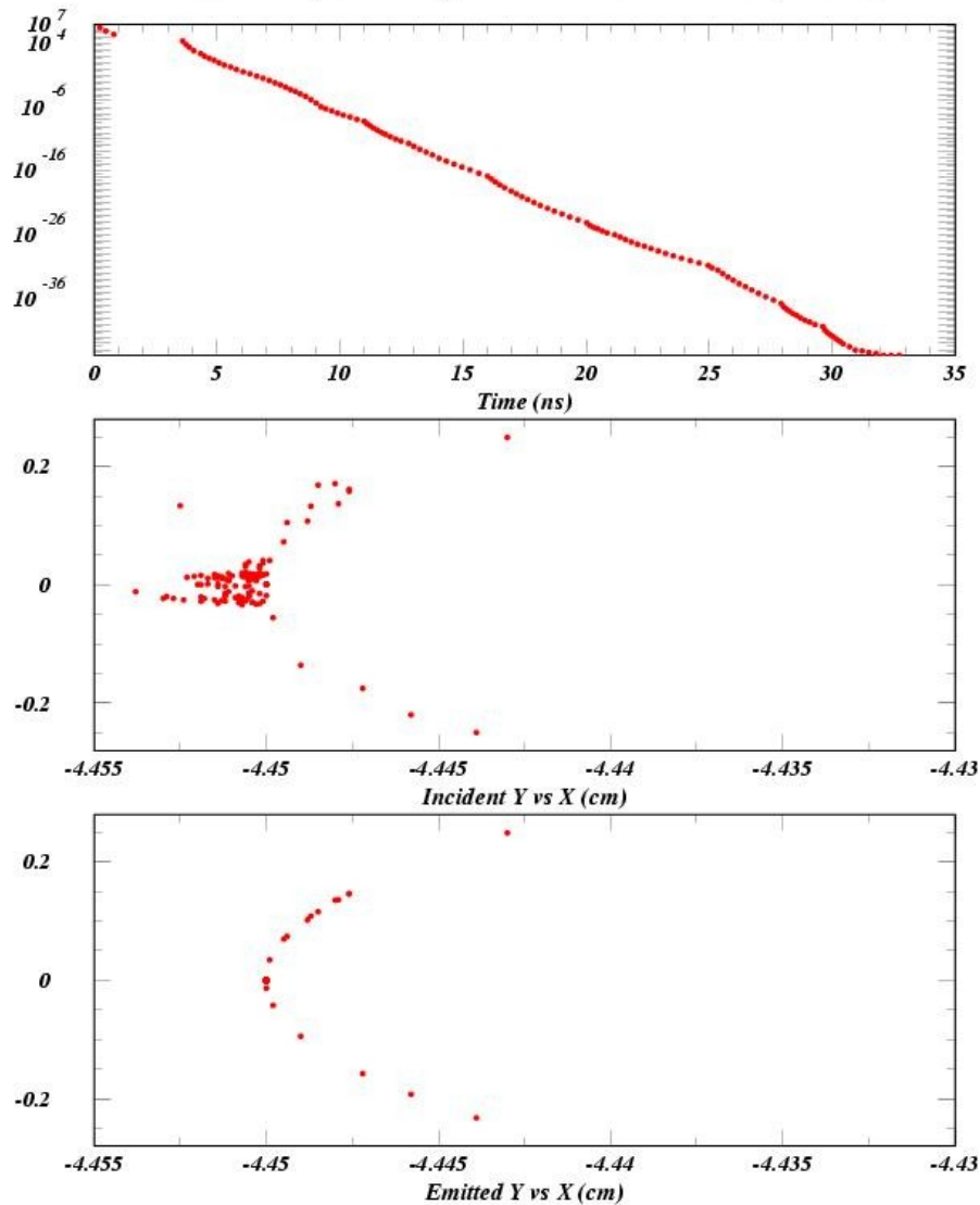
Resonant Loss of MP 38 in Job 10555: Time Evolution of Kinematics
