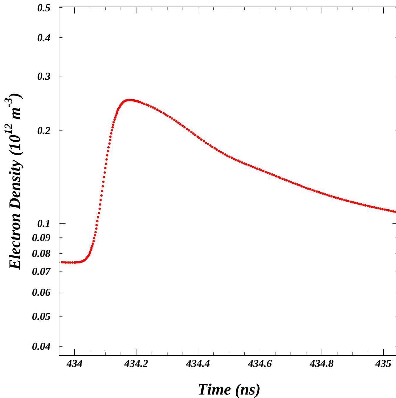
Job 41295: Beampipe-averaged Cloud Density ( 10^{12} \text{ m}^{-3} )
