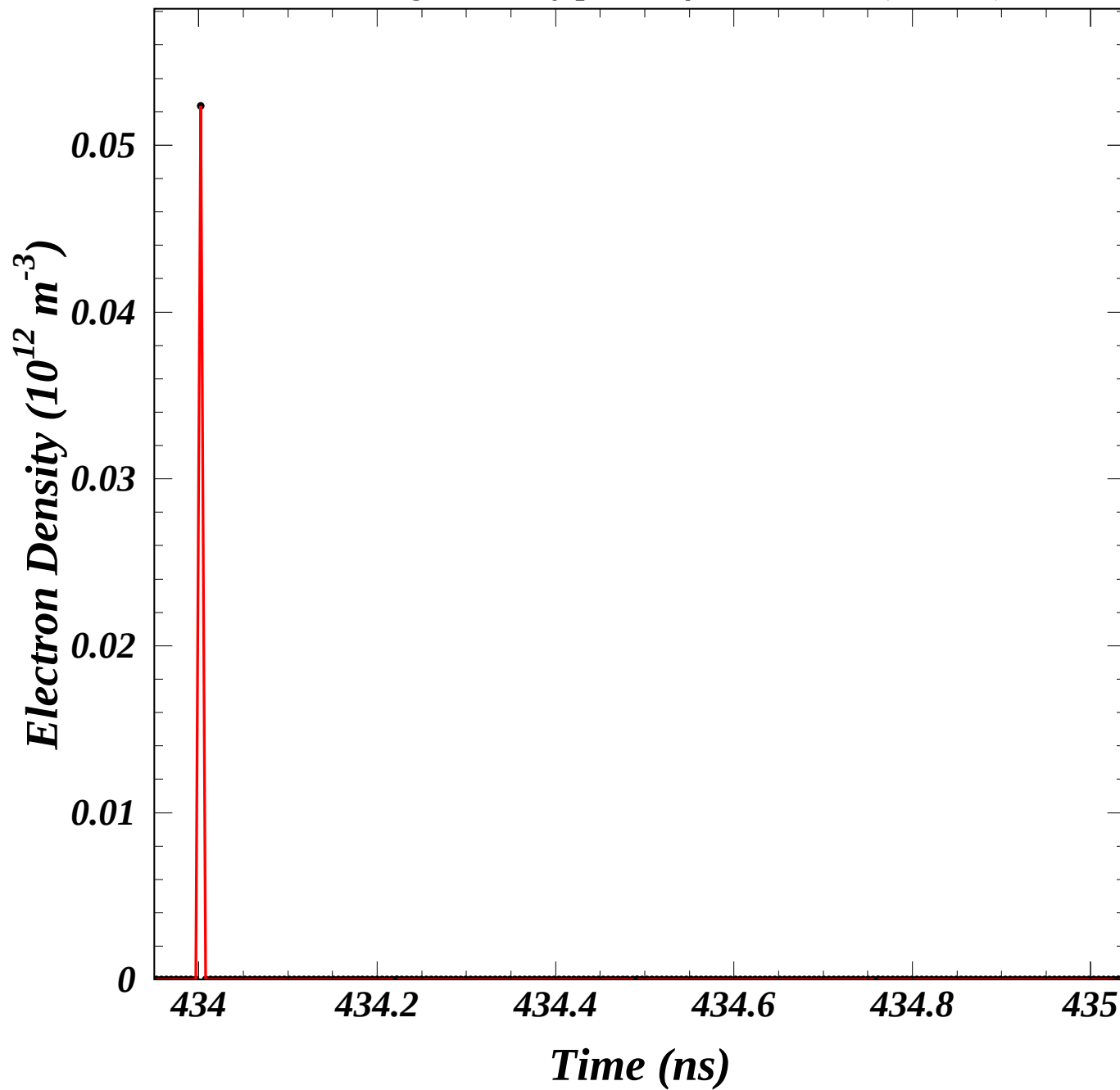
Central 100-sigma density prior to filled bunches ( 10^{12} \text{ m}^{-3} )
