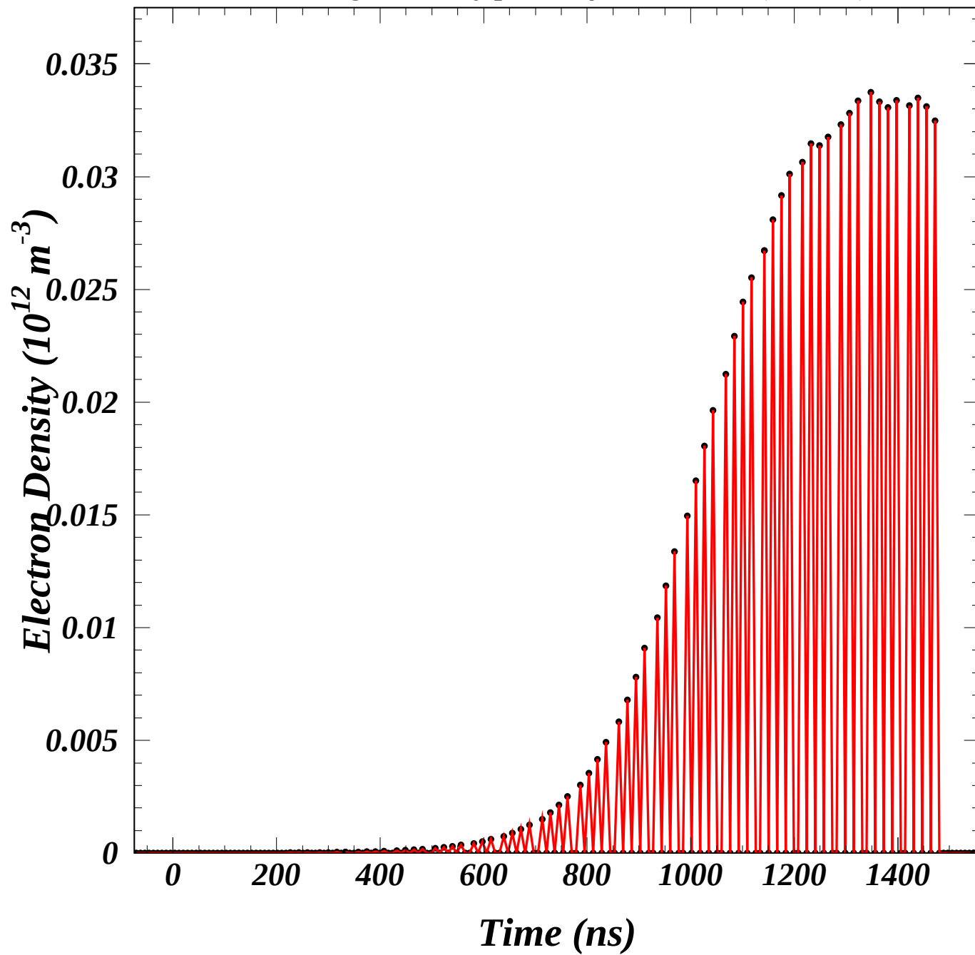
Central 20-sigma density prior to filled bunches ( 10^{12} \text{ m}^{-3} )
