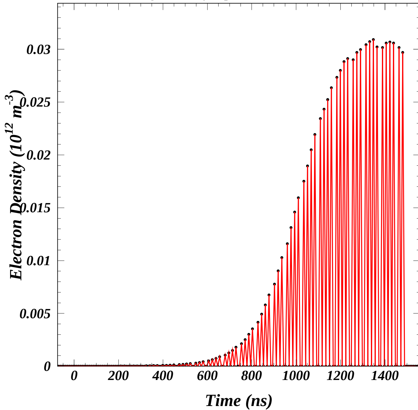
Central 20-sigma density at peak bunch current ( 10^{12} \text{ m}^{-3} )
