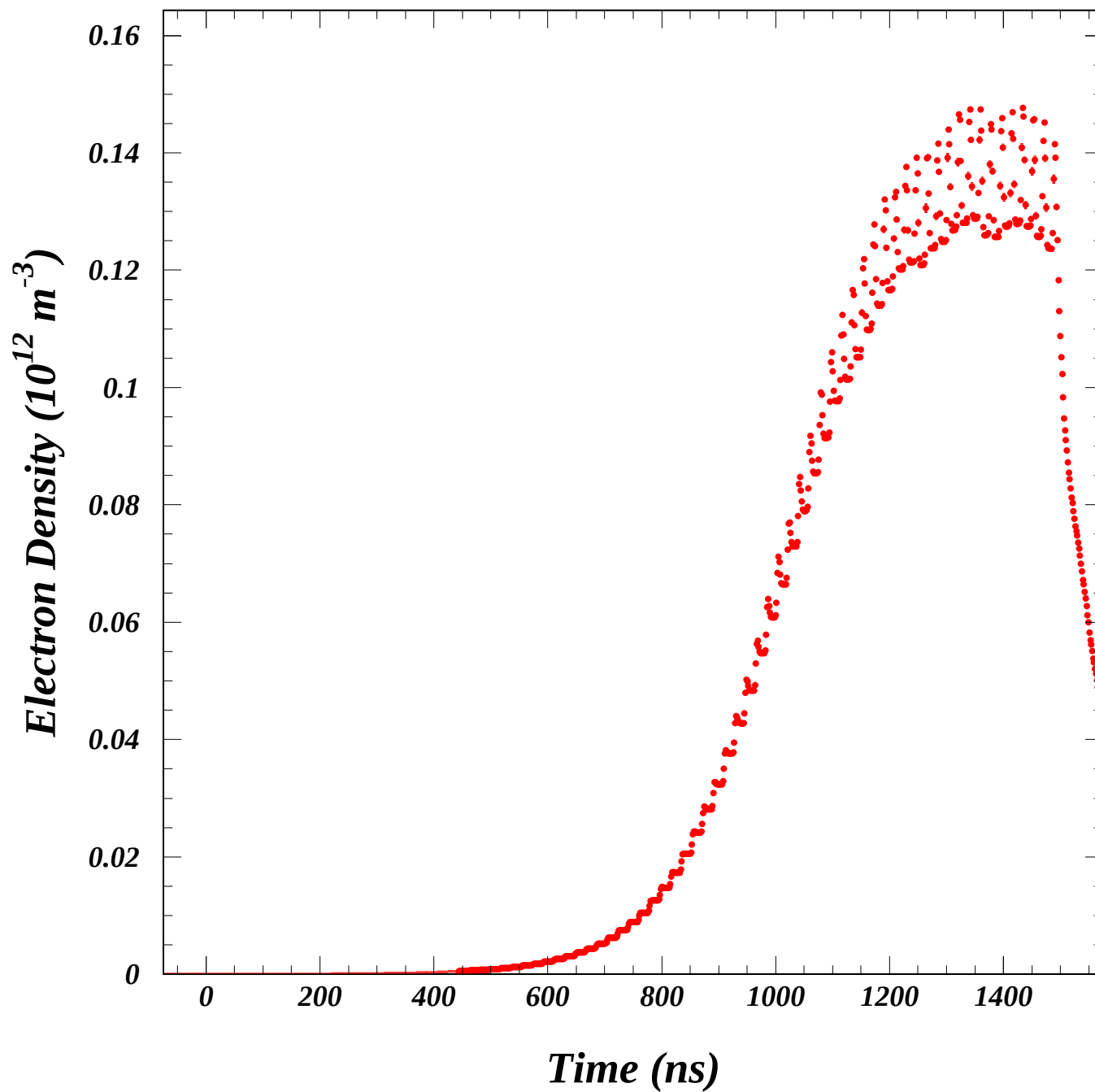
Job 51266: Beampipe-averaged Cloud Density ( 10^{12} \text{ m}^{-3} )
