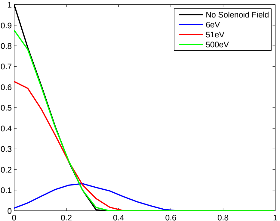
solenoid field at 20Gauss, no SEY
