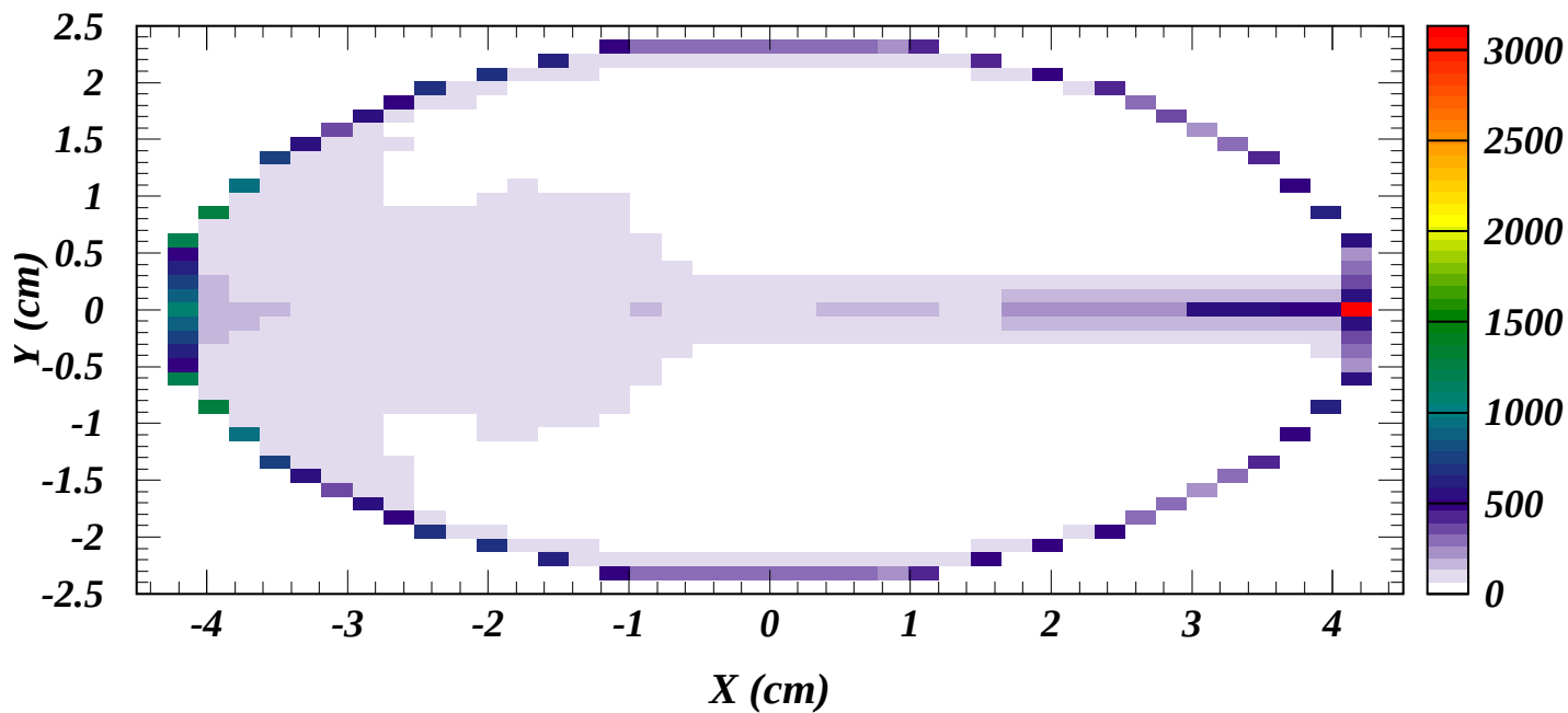
Job 33836: Cloud Density ( e/m^3 ) Averaged Over 40 ns
