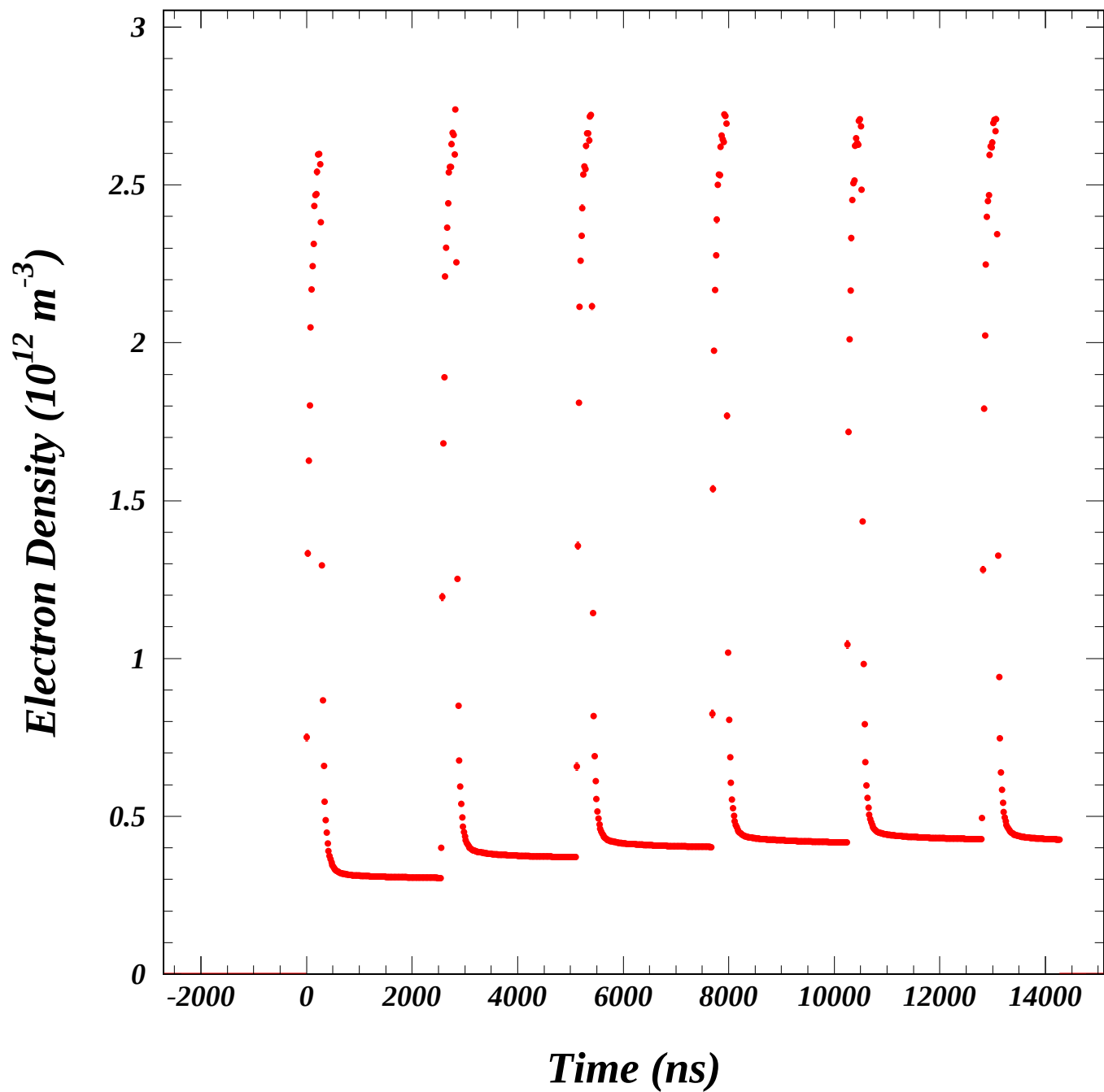
Job 34150: Beampipe-averaged Cloud Density ( 10^{12} \text{ m}^{-3} ) 12/10/08 11.19
