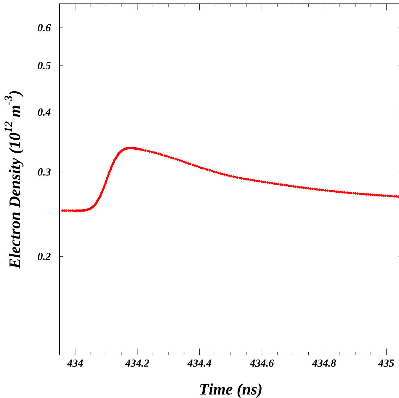
Job 41298: Beampipe-averaged Cloud Density ( 10^{12} \text{ m}^{-3} )
