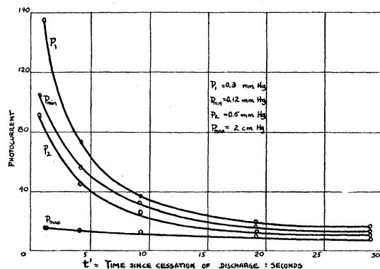
FIG. 4. Decay curves of un-outgassed aluminum. Various pressures.
