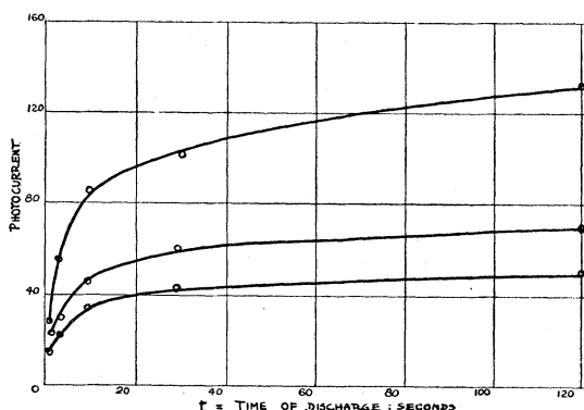
FIG. 3. Variation of sensitivity with time of discharge.
