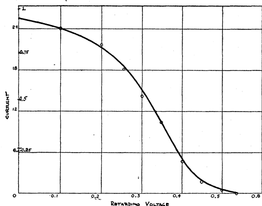
FIG. 11. Current-voltage curve for freshly evaporated aluminum.
