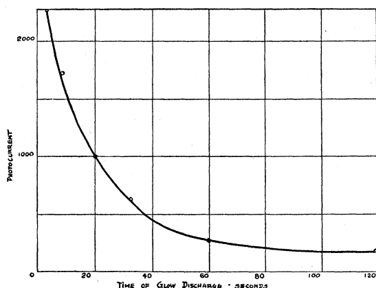
FIG. 7. De-sensitization of an air-sensitized aluminum surface.
