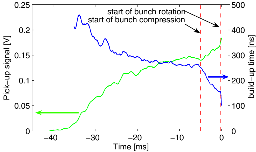
FIG. 11. (Color) Electron cloud buildup time (50% rise time) compared to the maximum electron signal at the end of the bunch train. As the bunch length decreases during the last tens of milliseconds before ejection, the EC signal increases while its buildup is accelerated. The bunch compression and rotation have a very distinct effect on both EC parameters.
