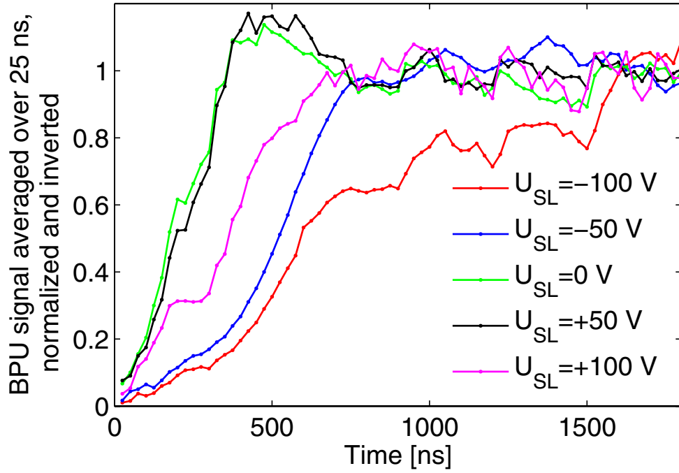
FIG. 10. (Color) Electron cloud buildup time for small clearing voltages without magnetic field. The raw signal from the pickup #2 was averaged for each bunch, normalized to the maximum signal value in the bunch train and inverted. Without magnetic field the curves closely follow exponentials.
