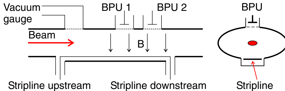
FIG. 1. (Color) Schematic view of the PS electron cloud experiment, comprising a shielded Penning gauge, two shielded button pickups (BPU), a stripline clearing electrode, and a dipole magnet (not sketched). Left: Longitudinal cut, right: transverse cut at the position of a BPU.
