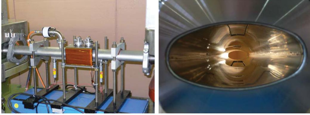
FIG. 2. (Color) Left: Picture of the new electron cloud experiment installed in PS straight section 98, containing two shielded button pickups, a shielded Penning gauge, a clearing electrode, and a small dipole magnet. Right: Downstream view into the vacuum chamber showing the stripline electrode at the bottom.
