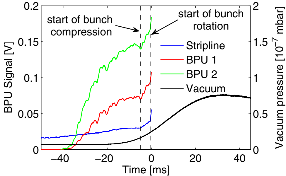
FIG. 6. (Color) The pickup signals (BPU 1 and BPU2) and the stripline peak signal (in arbitrary units) extracted from the raw data together with the vacuum pressure for the nominal LHC beam with 72 bunches. The EC becomes visible on the pickups about 40 ms before ejection, the vacuum gauge follows with a delay of about 30 ms.
