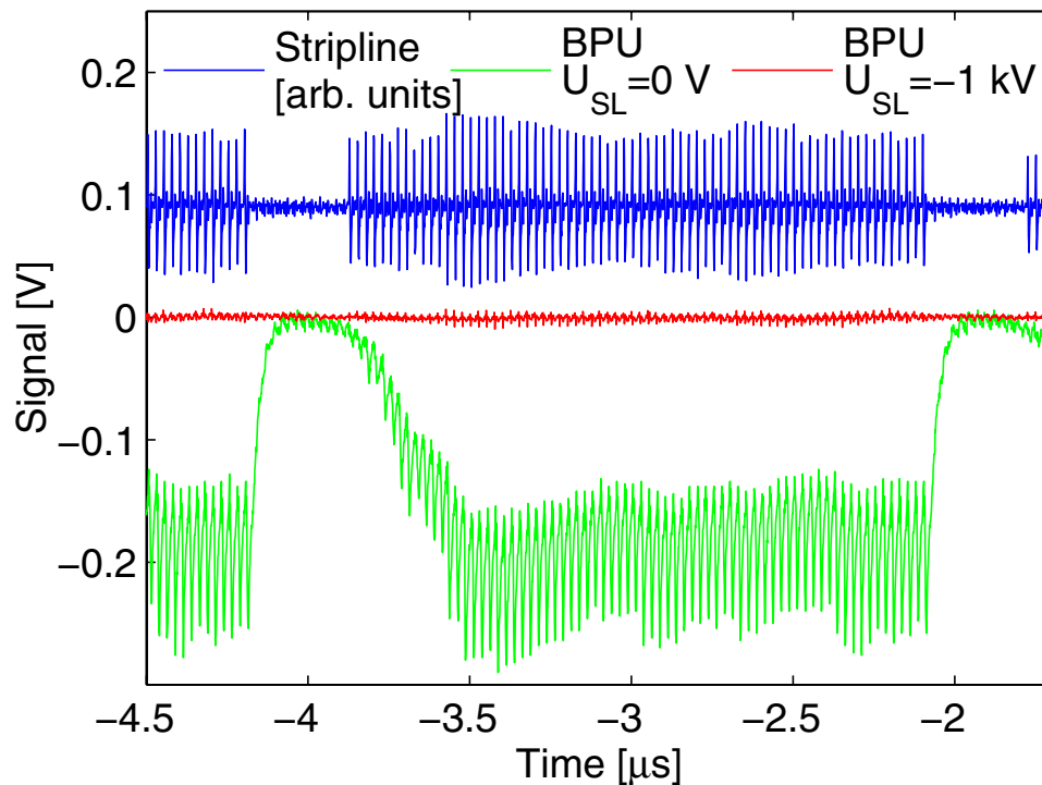
FIG. 8. (Color) The electron cloud was suppressed below the detection limit for large enough clearing voltages, e.g. U_{SL} = -1 kV, data from BPU 2 are plotted.
