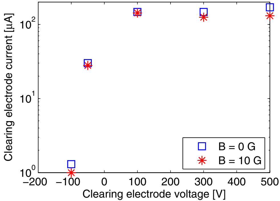
FIG. 14. (Color) The current drawn by the 40 cm long stripline electrode strongly depends on the polarity of the clearing voltage. For positive U_{\text{SL}} the current is rather large and essentially constant, while it is small for negative U_{\text{SL}} .
