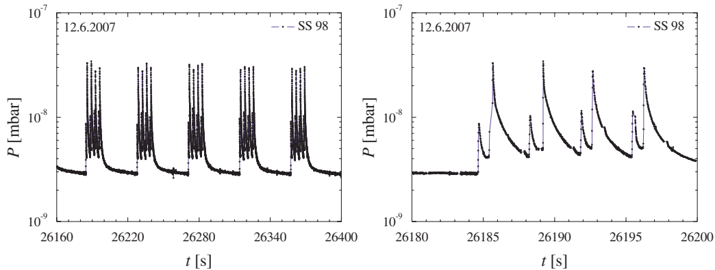
FIG. 3. (Color) Pressure rises in PS straight section 98 measured on 12/6/2007 at 21:38 during a PS supercycle that contained four nominal LHC beams. Right: Zoom into the pressure rise caused by 4 \times 72 bunches. The distance between the main peaks is 3.6 s, the smaller peaks appear about 0.8 s before.
