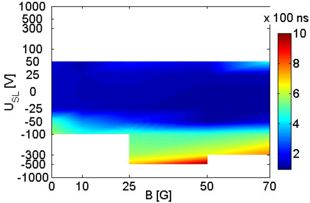
FIG. 12. (Color) Electron cloud buildup time measured with pickup #2 for the second last turn. The positions in the parameter space where the EC did not reach saturation are left blank in the plot. With magnetic field the buildup time shortens a bit, while it increases appreciably for negative clearing voltages.
