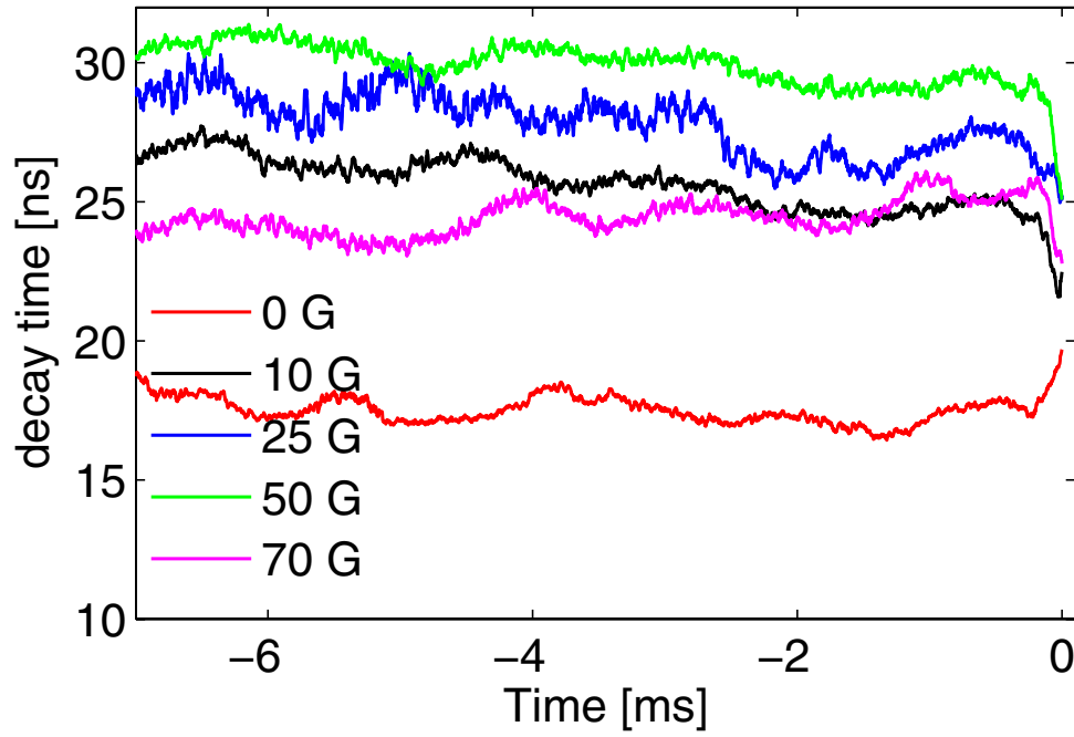
FIG. 13. (Color) Electron cloud decay time \tau during the last 7 ms of the PS cycle for different magnetic fields. The decay time is not very sensitive on the bunch length, but increases when a magnetic field is present.
