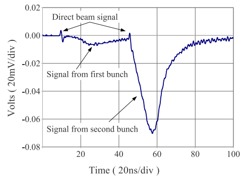
Figure 2: SPU signal with 2 bunches of 4.8 \times 10^{10} positrons each with bunches 36 ns apart. The beam energy is 2.1 GeV
