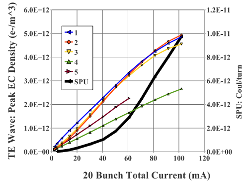
Figure 6: Comparison of SPU and TE Wave measurements for a 20 bunch train of positrons. The thick curve is the total charge deposited in the SPU in a single turn; the thinner, numbered curves are based on the TE Wave sidebands of five different resonances shown in Fig. 5.
