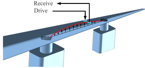
Figure 3: Standing waves are set up between ion pumps with longitudinal slots. Microwaves are coupled in/out of the beampipe using the electrodes of a beam position monitor. The resonances will be multiples of a half-wavelength.
