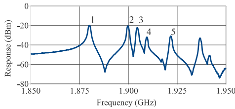
Figure 5: Above is the TE Wave response at 15E when resonantly excited. The sideband amplitudes of first five major peaks were used to generate Fig. 6 .
