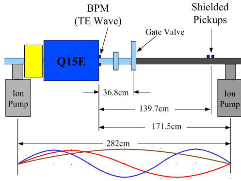
Figure 4: The SPU is located in a short test section of chamber where the vacuum surface has been coated with diamond-like carbon (the darker section in the sketch). The TE Wave region spans both the coated and uncoated sections of beampipe.
