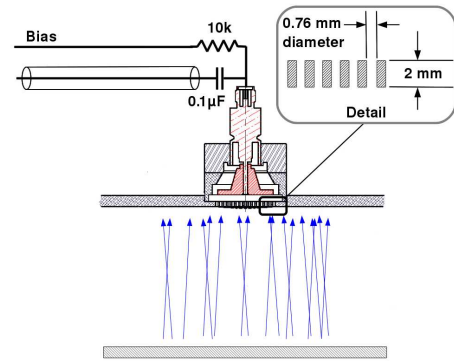
Figure 1: Sketch of Shielded Pickup (SPU)
