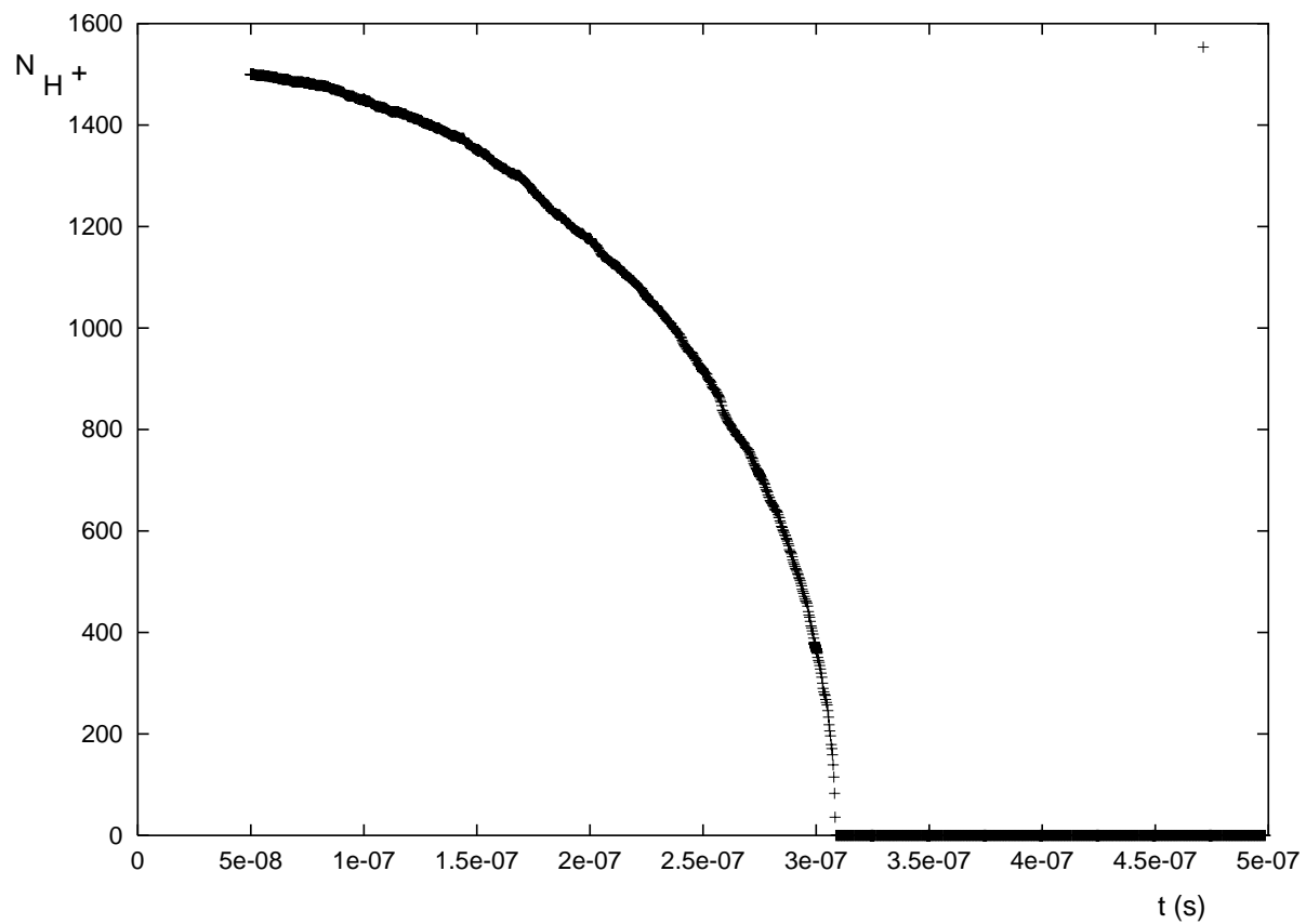
Figure 23: Number of ions in the beam pipe as a function of time. In this simulation we launched 1500 \text{ H}^+ ions at time t = 50 \text{ ns} .
