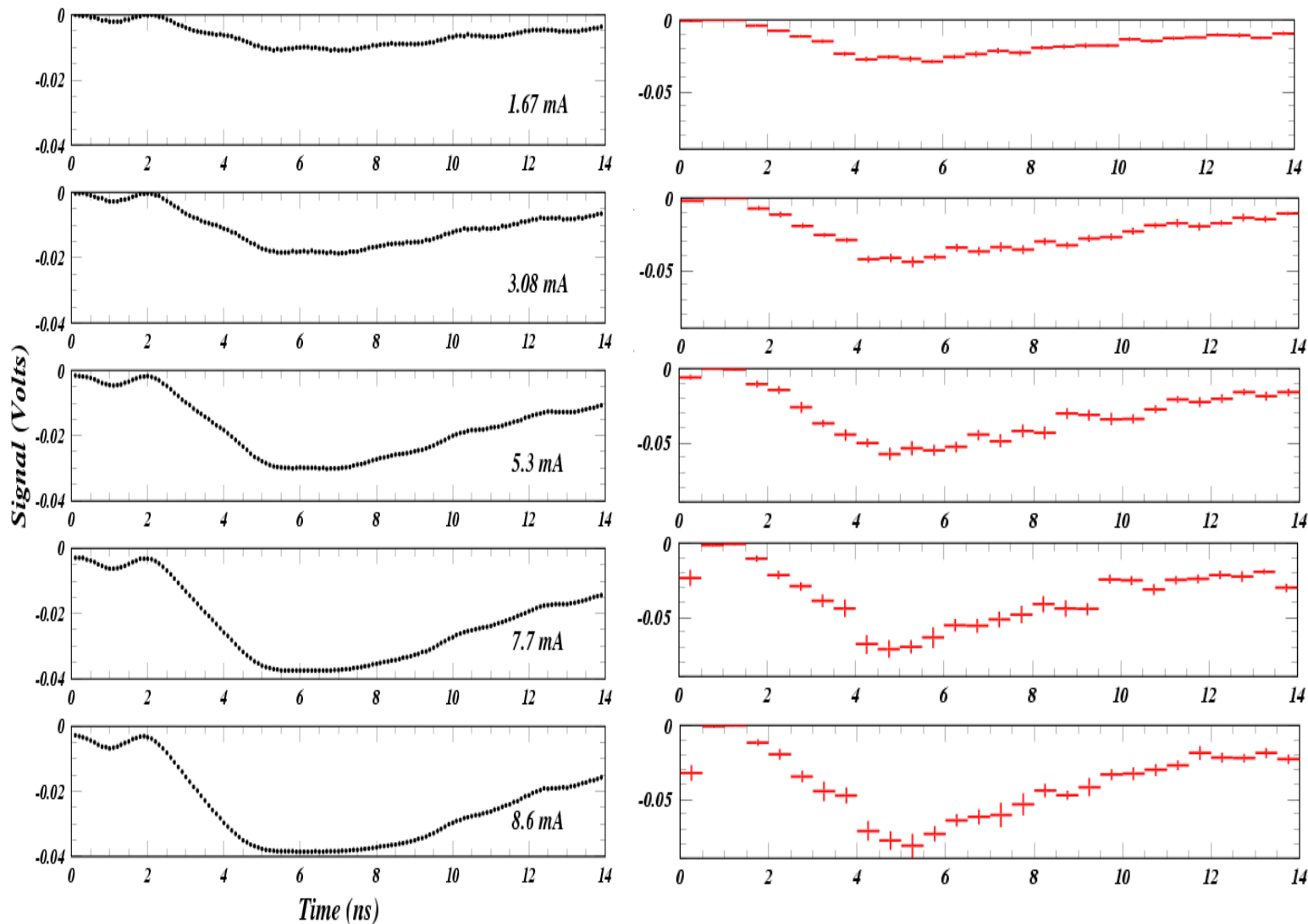
15E (TiN) SPU Measurements (3/16/2010, 5.3 GeV e^- , Button 2)
