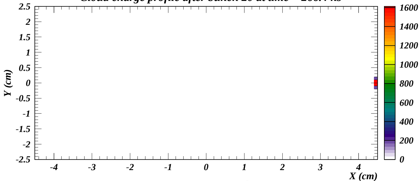
No energy cut: 199989 macroparticles, 1.27624e+10 \text{ e-}
