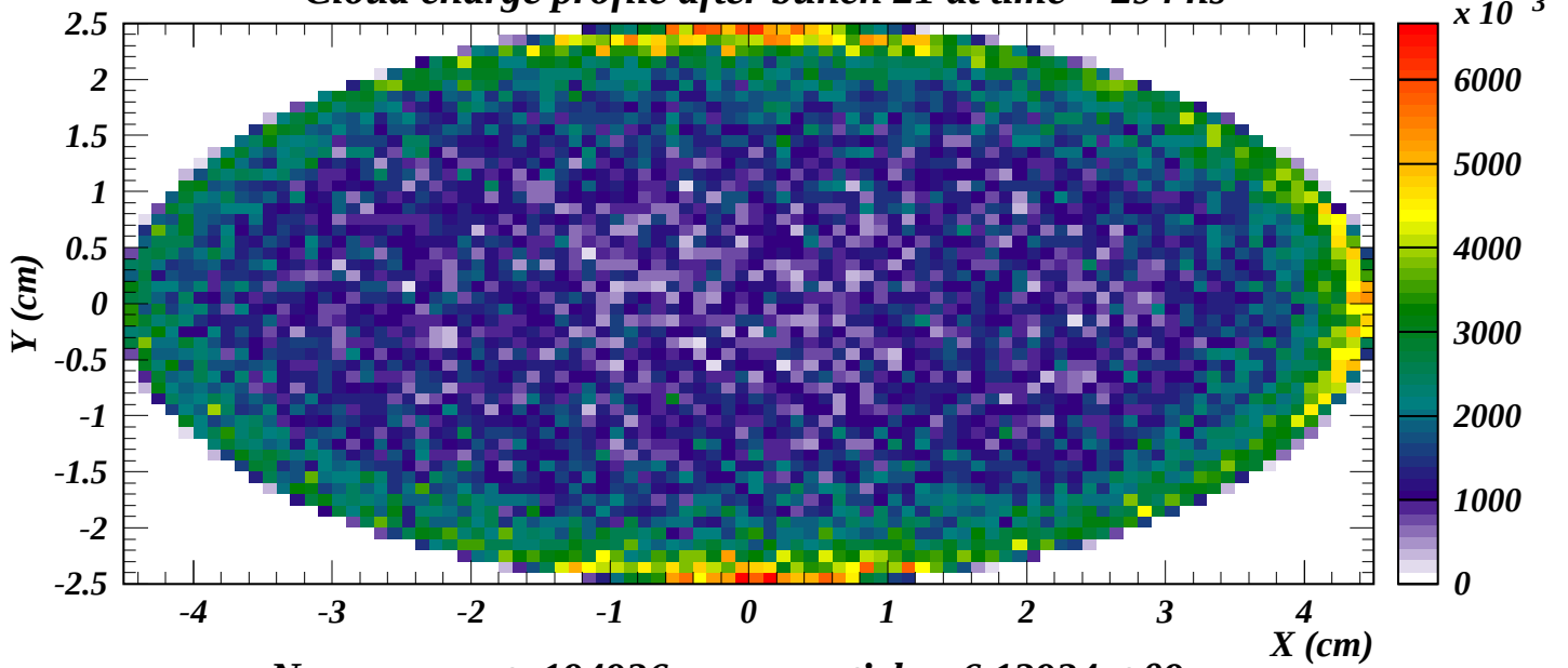
No energy cut: 194926 macroparticles, 6.13924e+09 e-
