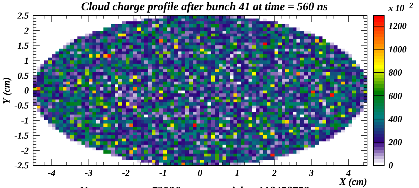
No energy cut: 73926 macroparticles, 118458752 e -
