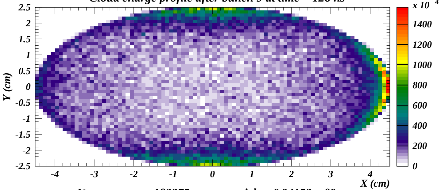
Cloud charge profile after bunch 9 at time = 126 ns
