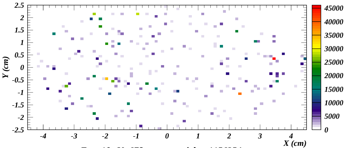
E_{\text{kin}} > 10 eV: 678 macroparticles, 1156354 e -
