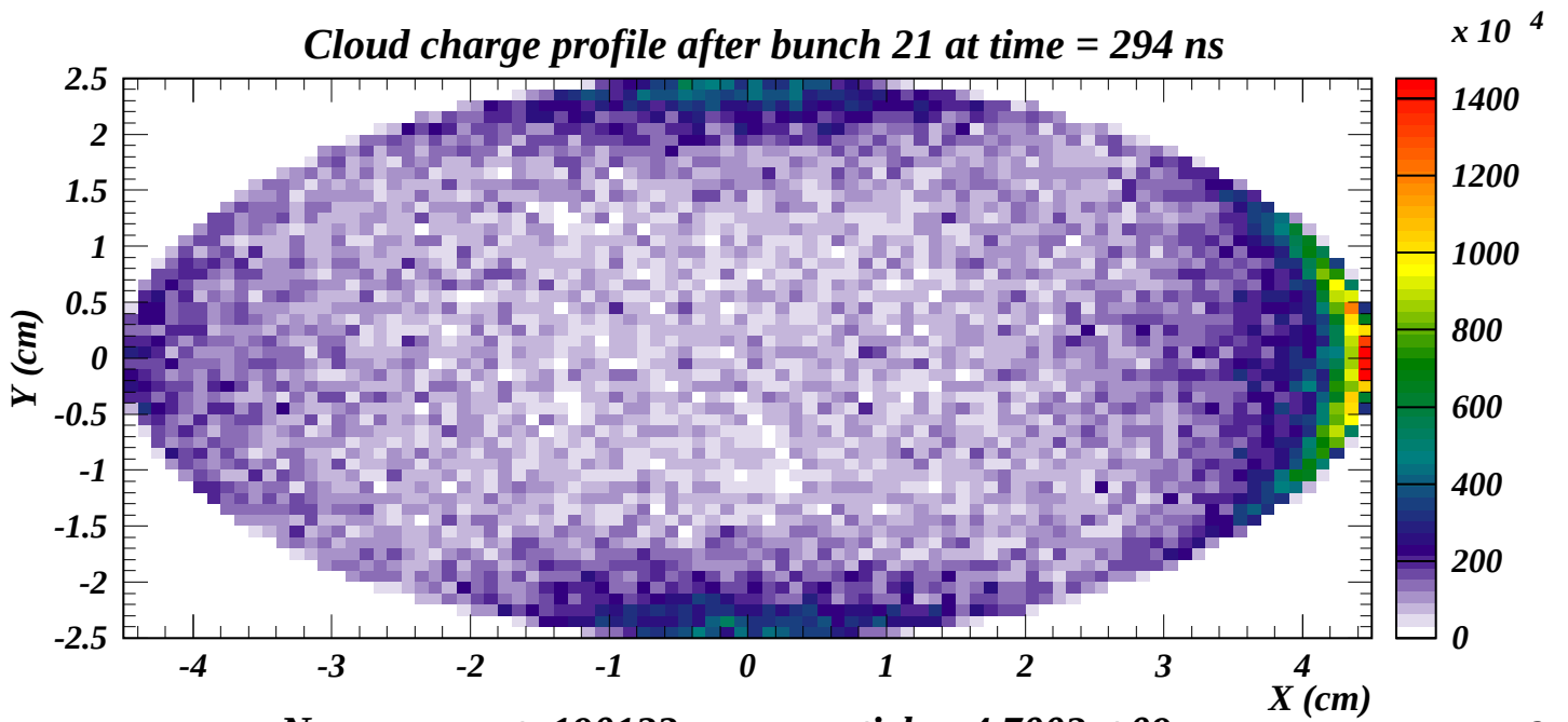
No energy cut: 190122 macroparticles, 4.7002e+09 e-
