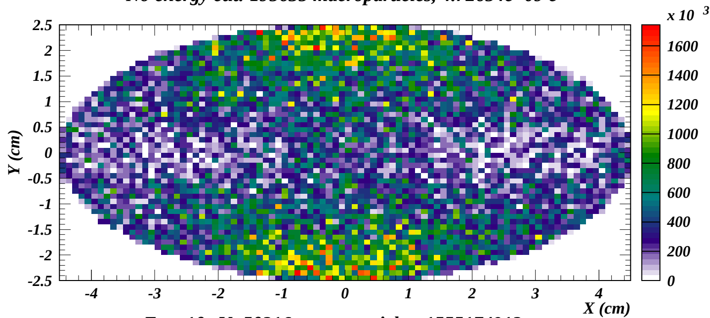
E_{kin} > 10 eV: 50216 macroparticles, 1555174912 e-
