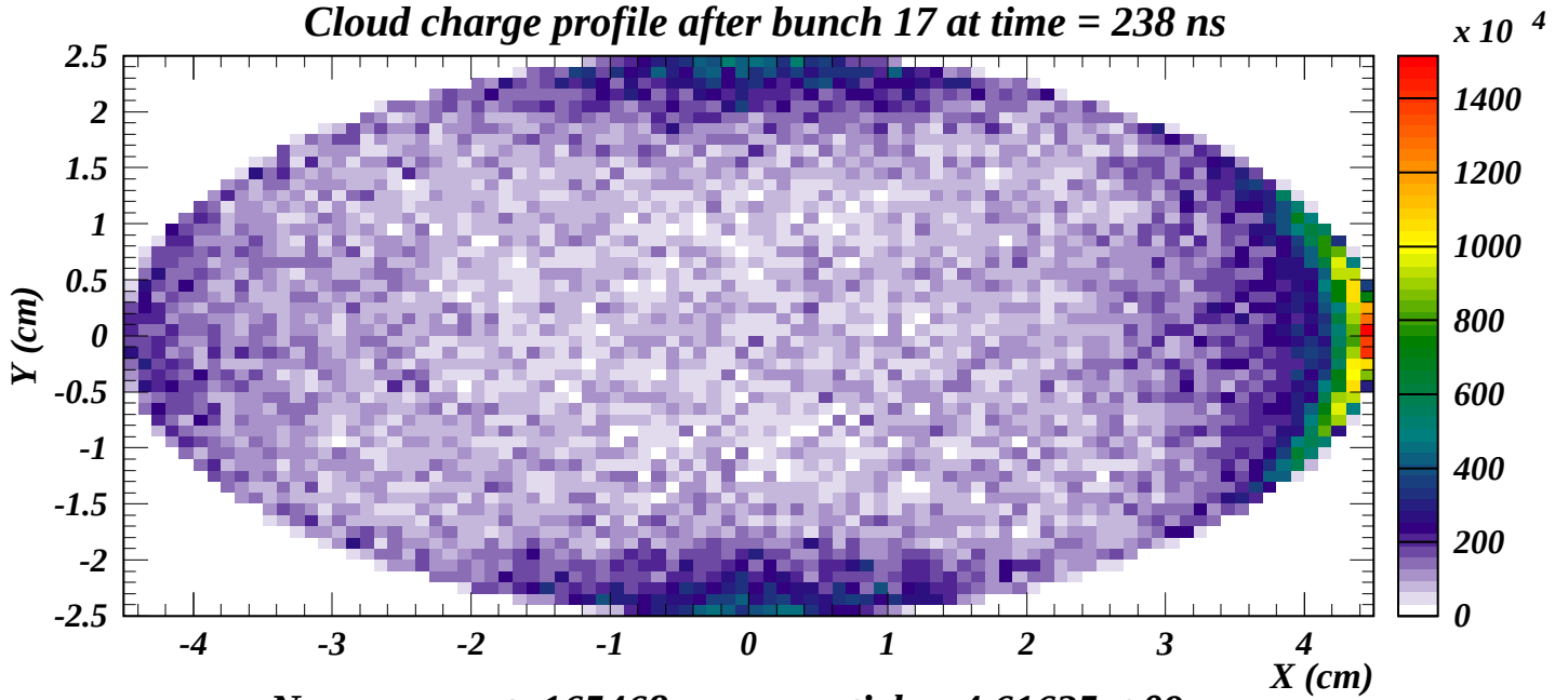
No energy cut: 165468 macroparticles, 4.61625 \times 10^9 \text{ e-}
