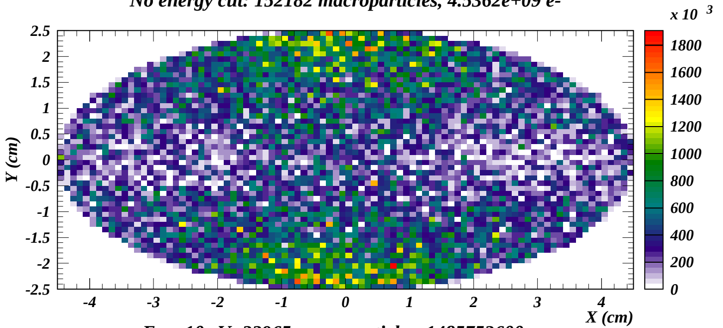
E_{\text{kin}} > 10 \text{ eV} : 32965 macroparticles, 1485753600 \text{ e-}
