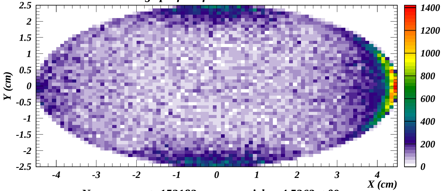
No energy cut: 152182 macroparticles, 4.5362e+09 \text{ e-}
