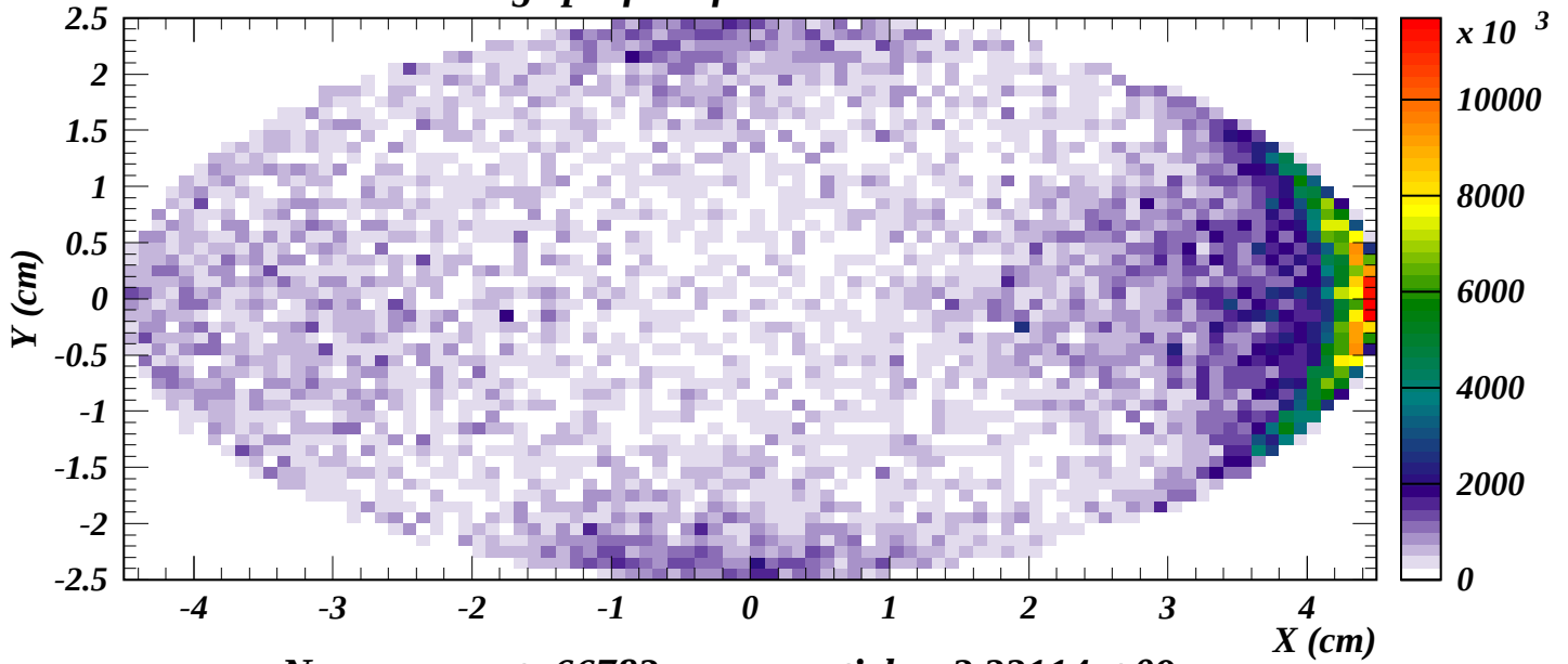
No energy cut: 66783 macroparticles, 2.33114e+09 \text{ e-}
