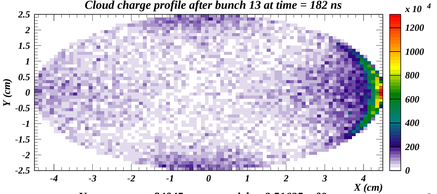
No energy cut: 84045 macroparticles, 2.51625e+09 \text{ e-}
