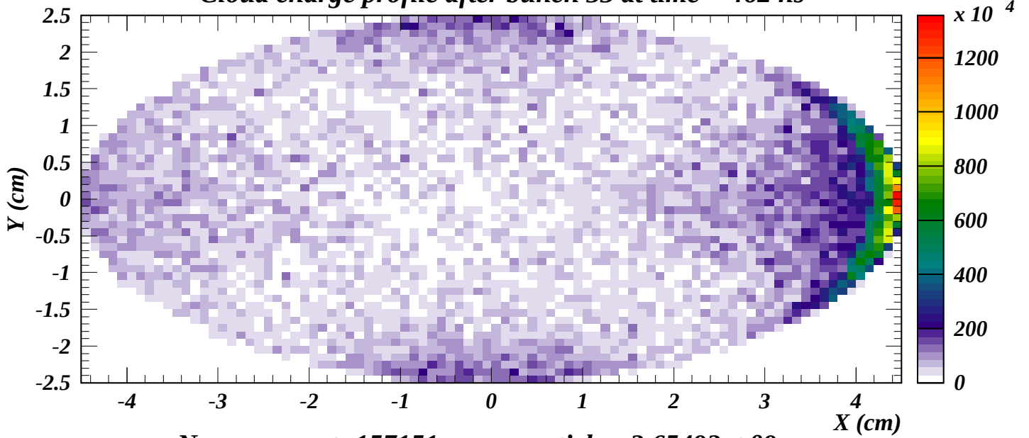
No energy cut: 157151 macroparticles, 2.65493e+09 e-
