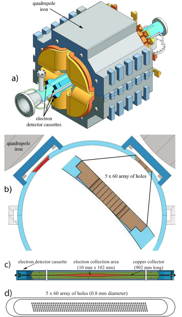
FIG. 1. a) Vacuum chamber equipped with electron detectors in the quadrupole magnet. b) Arrangement of two detectors in front of the magnet poles as seen from the positron arrival direction. c) Geometry of the copper electrode biased at 50 V to collect electrons entering through the pattern of holes in the beam-pipe shown in d). The rectangular region of the collector and the pattern of holes are each about 10 cm long.
