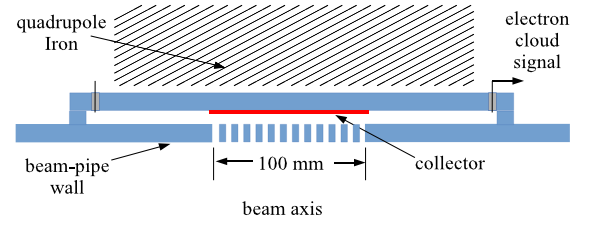
FIG. 2. Schematic cross section of the electron detector, which is located near the longitudinal center of the quadrupole magnet. The holes in the beam-pipe wall allow cloud electrons to reach the collector.
