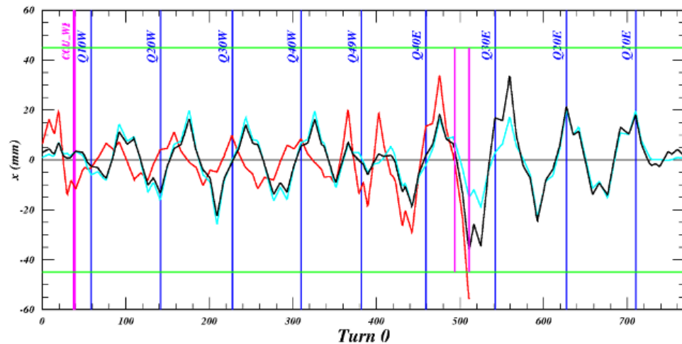
Job 2195: Horizontal Injected-Electron Orbit
