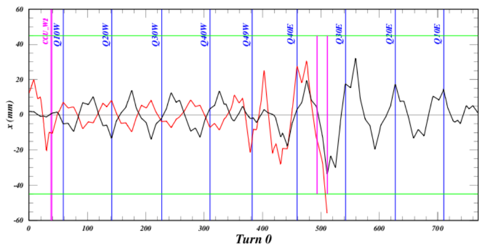
Job 2222: Horizontal Injected-Electron Orbit
