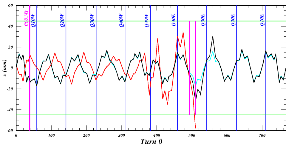
Job 2179: Horizontal Injected-Electron Orbit
