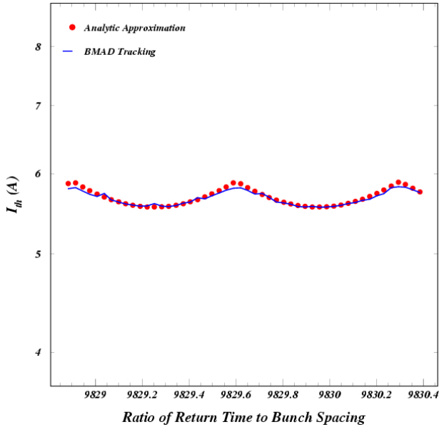
Figure 3: Comparison of the Bmad tracking result for the BBU instability threshold current for the full Cornell X-ray ERL optics with a single HOM in a single cavity, where the return time is much greater than the HOM decay time.
