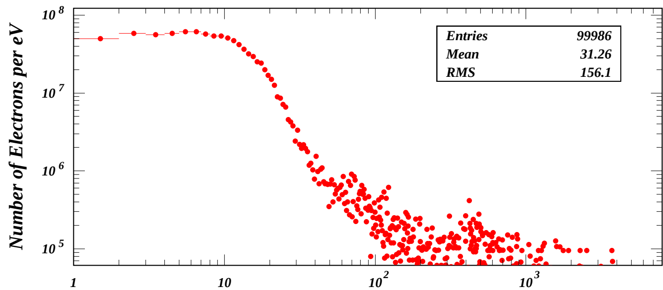
ECLOUD DR20100308_64_qua: Electron Cloud Charges Lost at Wall
