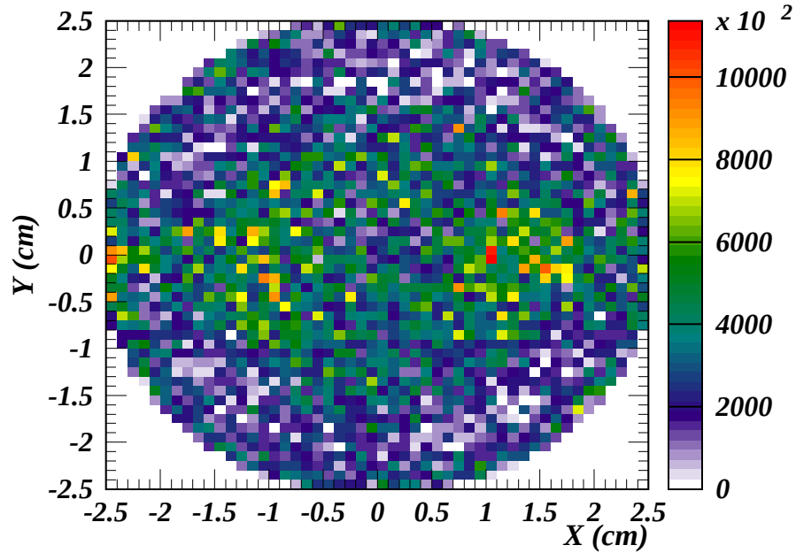
Cloud charge profile after bunch 21 at time = 126 ns
