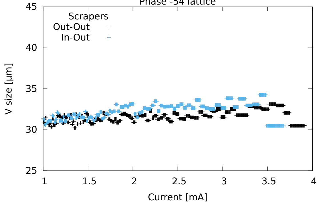
Phase -54 lattice
