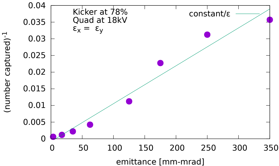
1/(Number captured) vs Emittance
