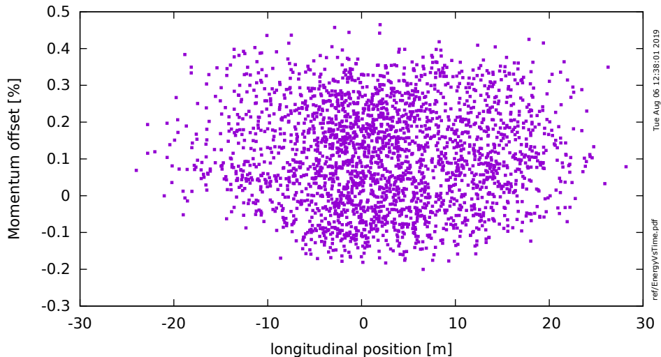
Longitudinal-Momentum phase space on first turn 20190614_191858
