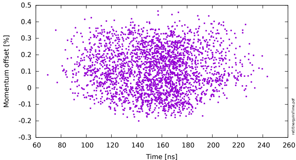
Time-Momentum phase space on first turn 20190614_191858
