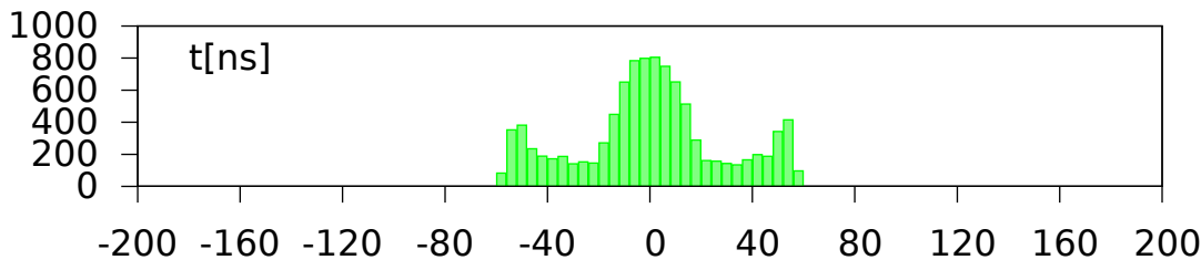
20180310_140300/DistStartInjLine_phase_space.dat
