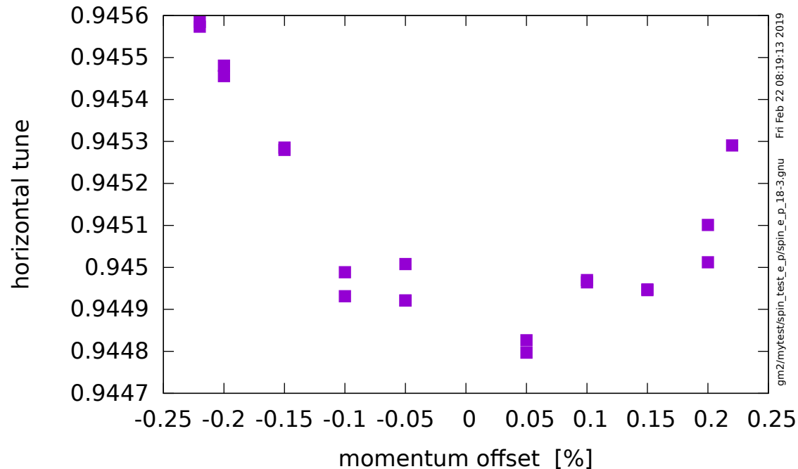
Horizontal tune vs momentum
