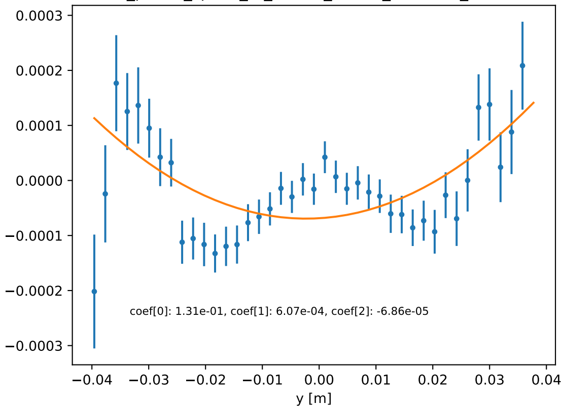
all_phase_space_at_70752_ns.dat_trimmed_sorted
