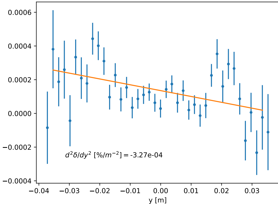
all_phase_space_at_56595_ns.dat_trimmed_sorted
