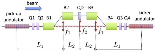
Fig. 1. Overview of the passive-OSC insertion beamline. The labels “Q,” and “B,” respectively refer to the quadrupole and dipole magnets and “ f_i ” represent the optical lenses. The solid blue (resp. undulatory red) line gives the electron (resp. light) trajectory.
