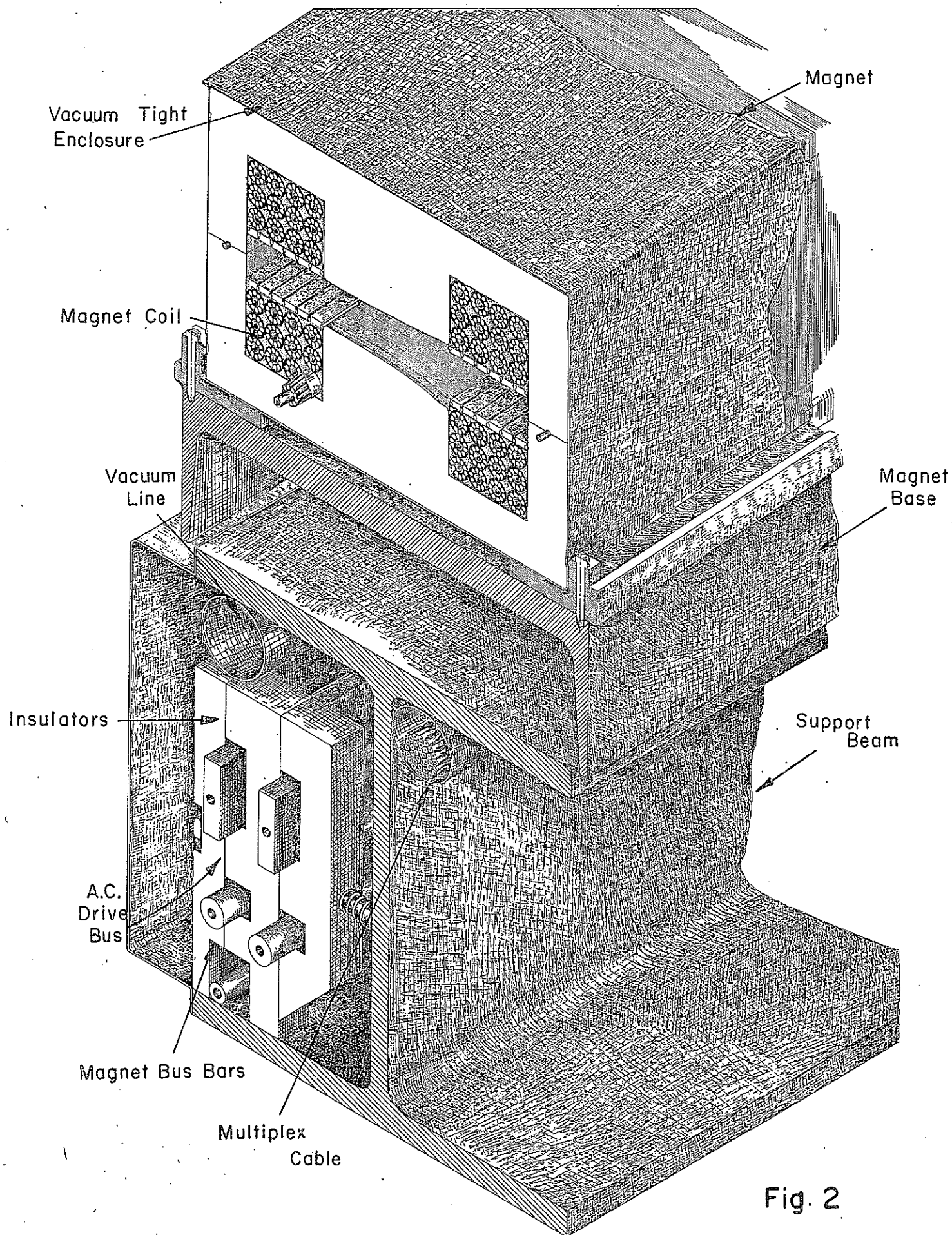
Cross-Section of a Synchrotron Magnet Unit
