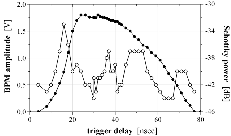
Figure 7.18. Measured Schottky power as the T_{\text{EL}} trigger delay is adjusted with respect to the intercepted bunch. The total Schottky power is plotted at each step, and should mimic the derivative (magnitude) of the pulse shape if timing jitter is significant.
