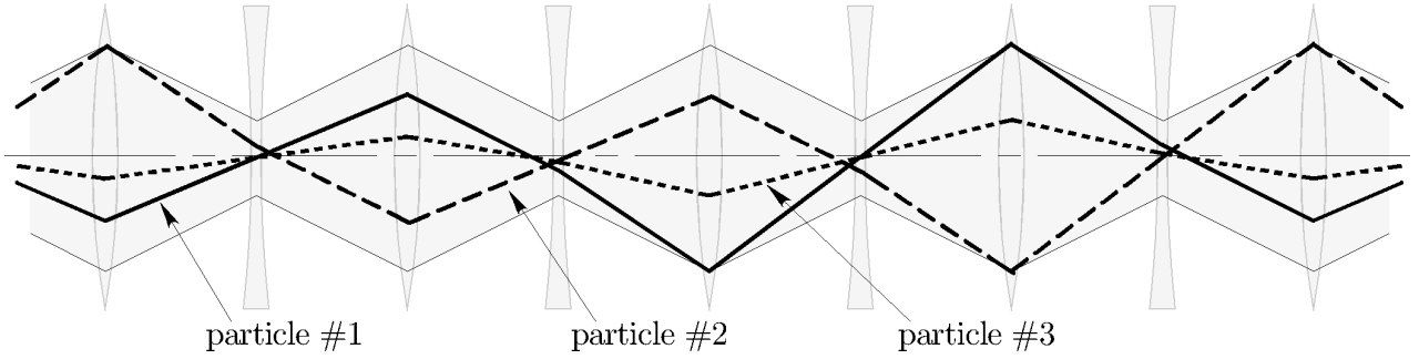
Figure 2.4. Illustration of three particles traveling through a FODO lattice. The envelope, proportional to \sqrt{\beta(z)} , is shown in grey. The first two particles have the maximum amplitude but different phases, so they brush against the envelope at different positions. The third has a much smaller amplitude, and deviates little from the central orbit.
