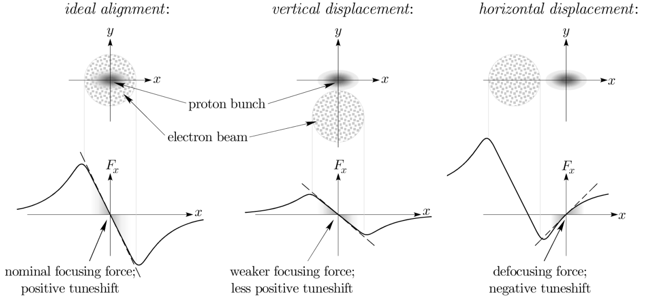
Figure 7.3. Illustration of how displacements can cause positive or negative tune shifts. A proton bunch centered on the electron beam feels a maximum positive tuneshift (left). A vertical displacement generates a lesser tuneshift (middle), but a horizontal displacement can create a negative tuneshift (right).
