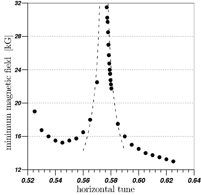
Figure 6.5. Minimum field strength as the horizontal tune is scanned across the vertical tune. In this case, \nu_y = 0.575 , \nu_s = 0.001 , \Delta\nu = -0.01 , N_{\bar{p}} = 6 \times 10^{10} , and \sigma_{\bar{p}} = 0.7 mm.
