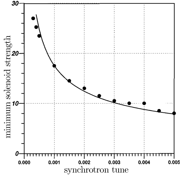
Figure 6.3. Minimum magnetic field strength versus the synchrotron tune. The data shown was generated with \nu_x = 0.585 , \nu_y = 0.575 , \Delta\nu = -0.01 , N_{\bar{p}} = 6 \times 10^{10} , and \sigma_{\bar{p}} = 0.7 mm. A fitted function B_{\min} = k\Delta\nu_s^{-1/2} produced a constant k = 0.557 and is also drawn.
