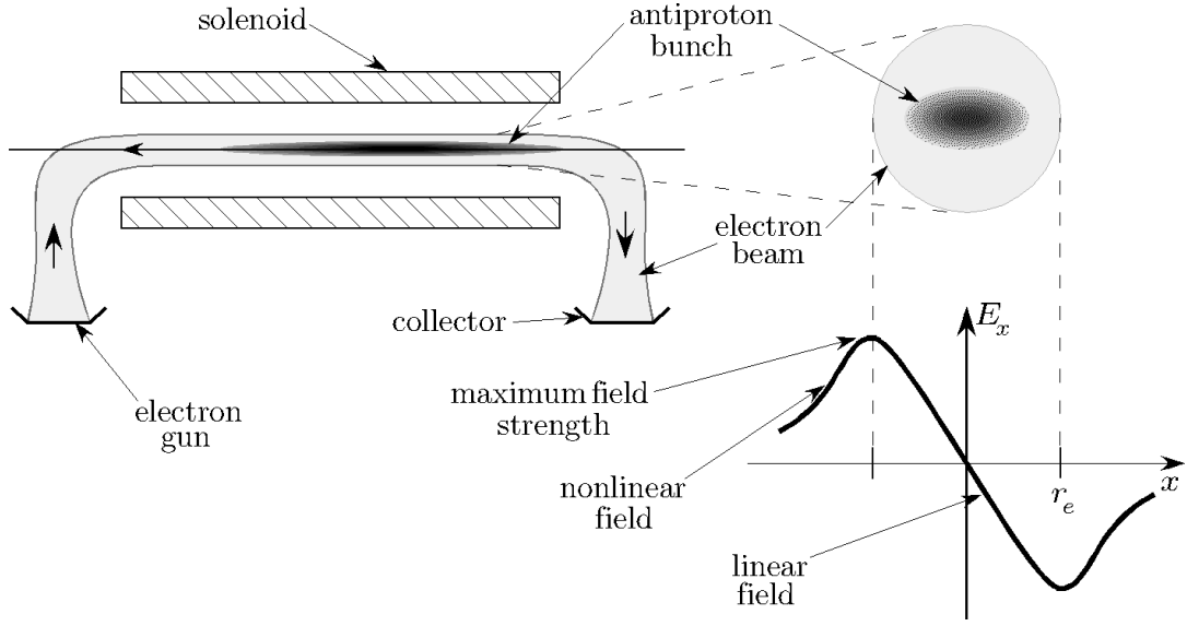
Figure 3.2. Cartoon of the interaction of the electron beam and the antiprotons. The protons pass significantly far away from the electron beam that they feel little effect. It is assumed for now that the electron beam profile is flat and that its radius is larger than that of the antiproton bunch.
