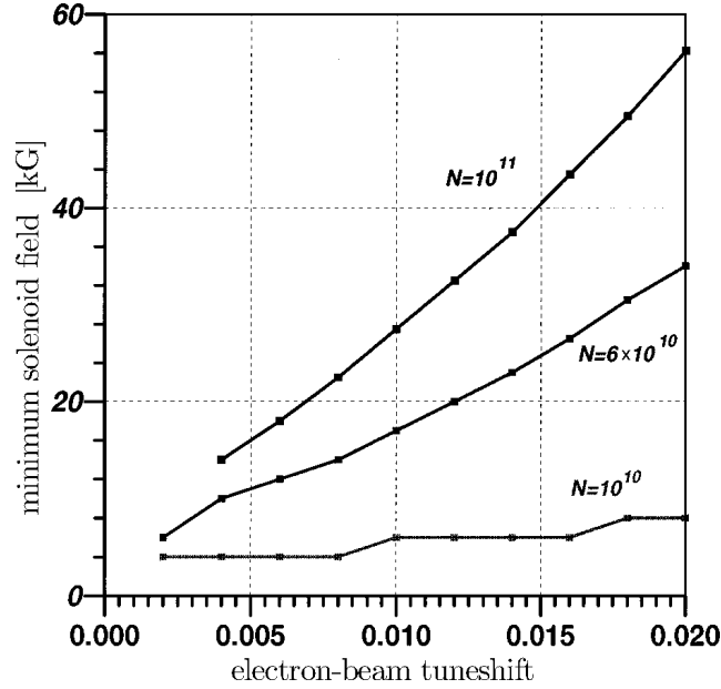
Figure 6.2. Minimum field strength in the T EL solenoid to prevent TMCI. The simulation gives sensible results; the approximately linear dependence on the number of antiprotons and on the tuneshift is apparent. The staircase appearance of the N_{\bar{p}} = 1 \times 10^{10} case stems from the limited number of iterations performed. The linear dependence relates well to the linear dependence of B_{\min} on N_{\bar{p}} and the total tuneshift \Delta\nu = \sqrt{\Delta\nu_x \Delta\nu_y} expressed in Equation 3.13. In these simulations, \nu_x = 0.585 , \nu_y = 0.575 , \nu_s = 0.0012 , and \sigma_{\bar{p}} = 0.7 mm.
