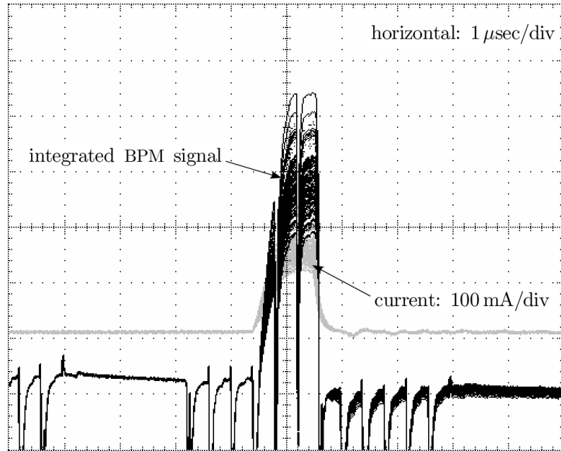
Figure 7.19. Trace of the T_{EL} agitating two antiproton bunches. While the individual signals are overlaid, the light grey is the current from the cathode and the black is the BPM plate signal (integrated once). The multiple traces typify the large pulse-to-pulse variations.
