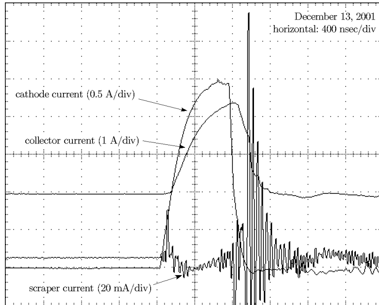
Figure 5.28. Oscilloscope trace illustrating a typical pulse of cathode, collector, and scraper currents. The cathode and collector currents peak current of at approximately 2.45 A. The time delay is simply the amount of time it takes for the electron beam to travel the entire path from cathode to collector, plus another 1.5 m of additional cabling to the high-voltage enclosure.
