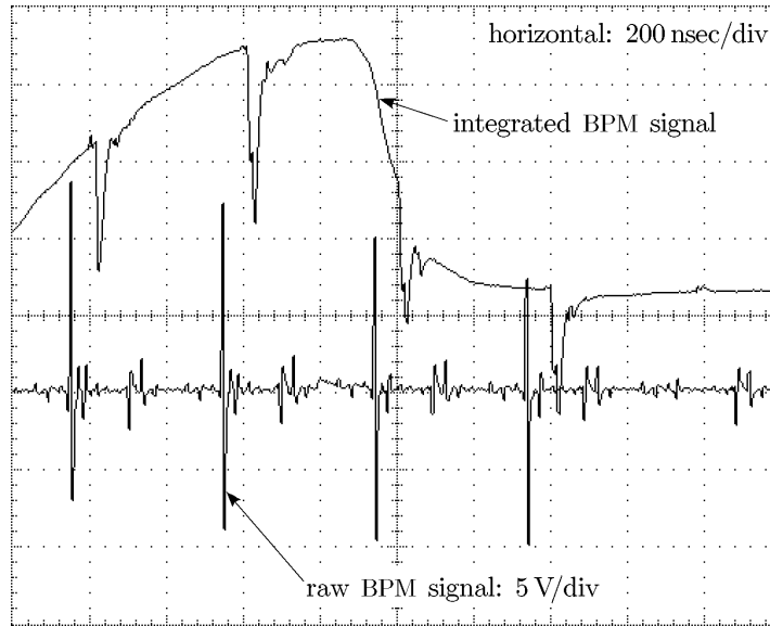
Figure 7.14. Display of the bunches passing through the T_{\text{EL}} electron beam pulse. The upper trace shows an integrated BPM plate, the lower shows a raw BPM plate signal. The slowly rising and falling electron beam intercepts several proton and antiproton pulses, but only the antiproton pulses are transversely centered on the electron beam.
