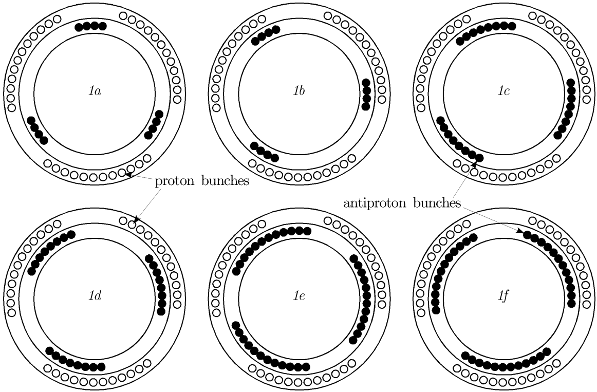
Figure 1.3. Illustration of loading antiprotons into the Tevatron. The hollow circles represent protons, which are loaded first. In 1a , the first four antiproton bunches (filled circles) in each train have been injected into the abort gap. These bunches are advanced forward ( cogging ) in 1b , before another batch of four bunches is injected in 1c . The antiprotons are again advanced ( 1d ), the final batch is injected ( 1e ), and everything is advanced so that proper bunch can collide at CDF and DØ.
