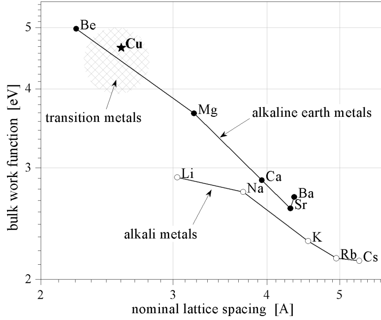
Figure 4.3. Correlation between lattice spacing and work function. Different elements will form different crystalline structures, and different faces will yield different atomic planar densities; hence the lattice spacing is not perfectly comparable. The alkali metals show a strong logarithmic connection between spacing and the work function, as do the alkaline earth metals. The transition metals tend to have similar behavior; most of them huddle in the region around copper.
