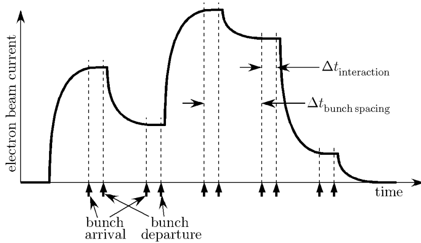
Figure 3.3. Cartoon of ramping the T E L current between adjacent antiproton bunches. The ramp shape mimics the real shape as observed in Figure 5.28. The events along the time axis indicate when the head of an antiproton bunch first enters one end of the electron beam and when the tail finally exits the other; this duration is much longer than just the length of the antiproton bunch. It is important that the electron-beam current reaches the desired level and is stable there early enough to ensure that the entire interaction length has a defined charge density.
