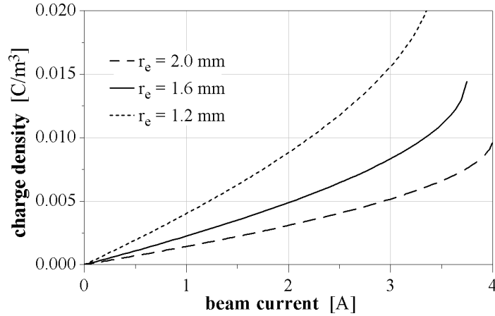
Figure 4.12. Charge density at the center of an electron beam. The density bends upward due to the slowing of the electrons immersed in the large current. A decrease in the beam radius drastically increases the density, but it also increases the dependence on accurate alignment.
