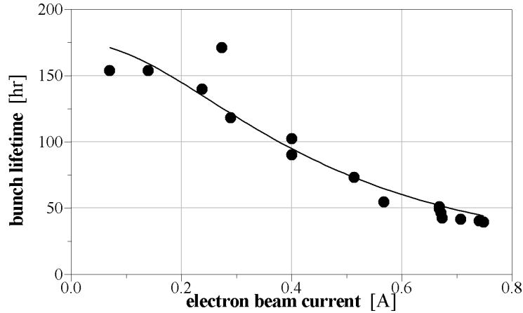
Figure 7.9. Typical bunch lifetime of a single proton bunch interacting with the TEL electron beam. This data is for the flattop gun, and it singlehandedly indicates the necessity of switching to a smoother beam profile, as discussed in Section 3.4. Shortly after this problem was noted, the Gaussian gun was installed.
