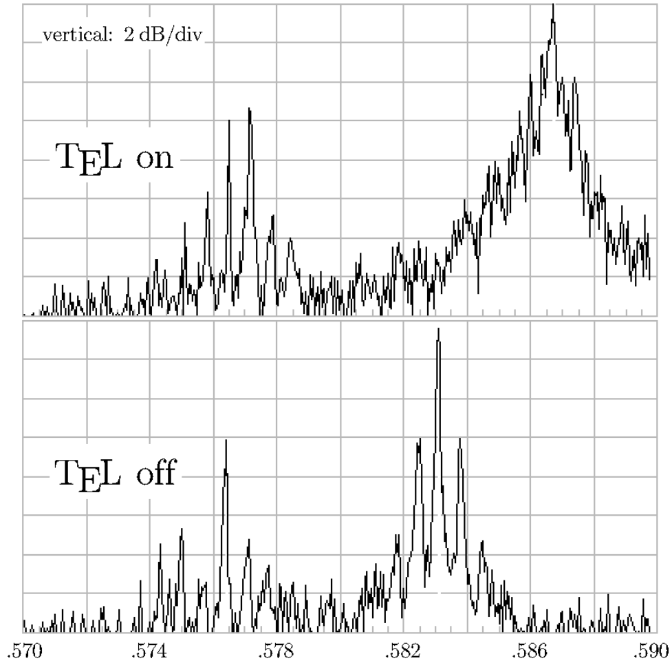
Figure 7.1. Horizontal Schottky spectra with and without the T_{EL} acting on a single proton bunch. The left set of peaks is crosstalk from the vertical tune, while the right set are the significantly changed horizontal tune.
