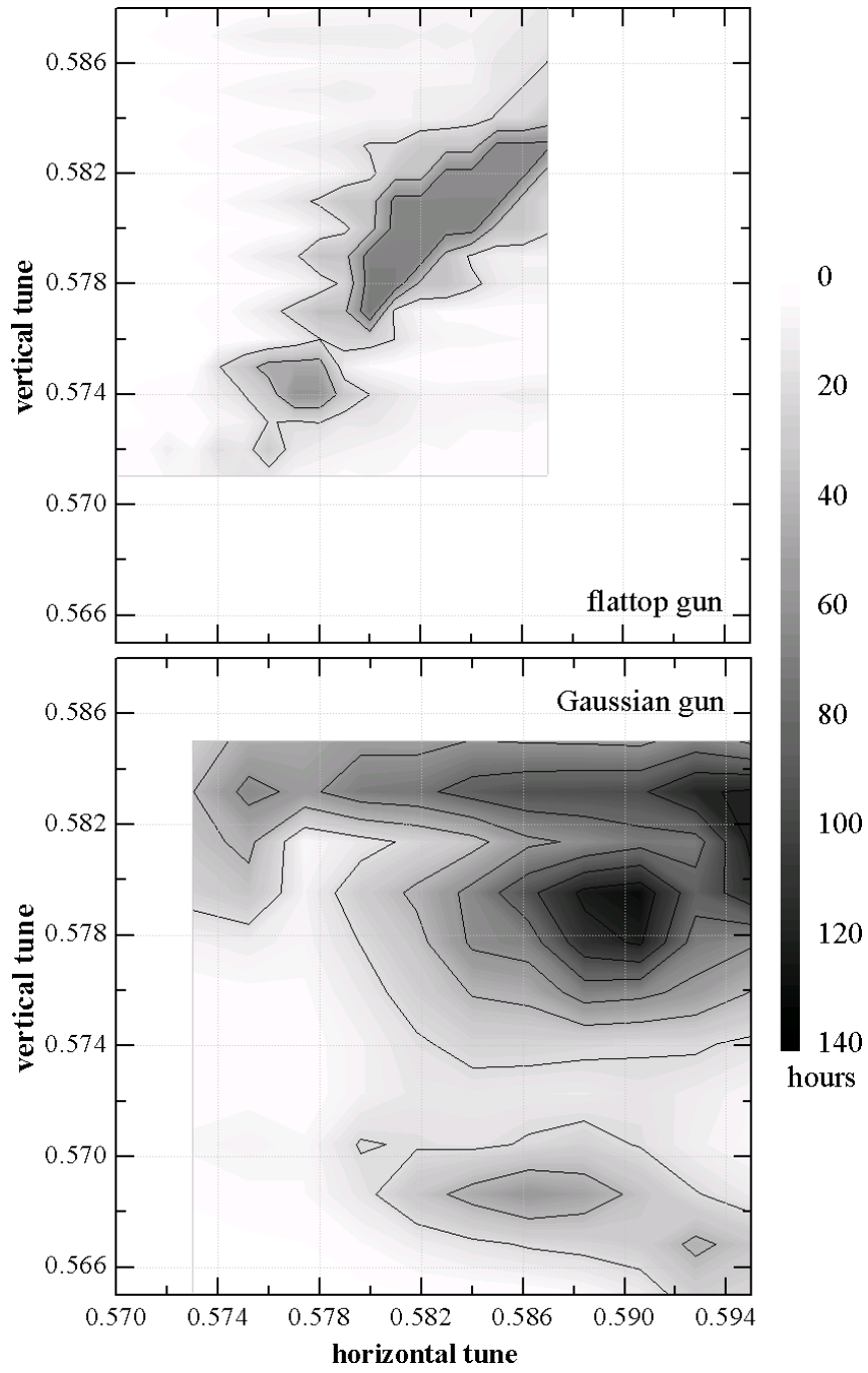
Figure 7.11. Scans of working points with the T_{\text{EL}} shifting the Tevatron tune. Both of the flattop (top) and Gaussian (bottom) guns were set to push the tune of a single proton bunch by about 0.004 horizontally. Data points generating these greyscale maps were taken at 0.002 intervals in each direction.
