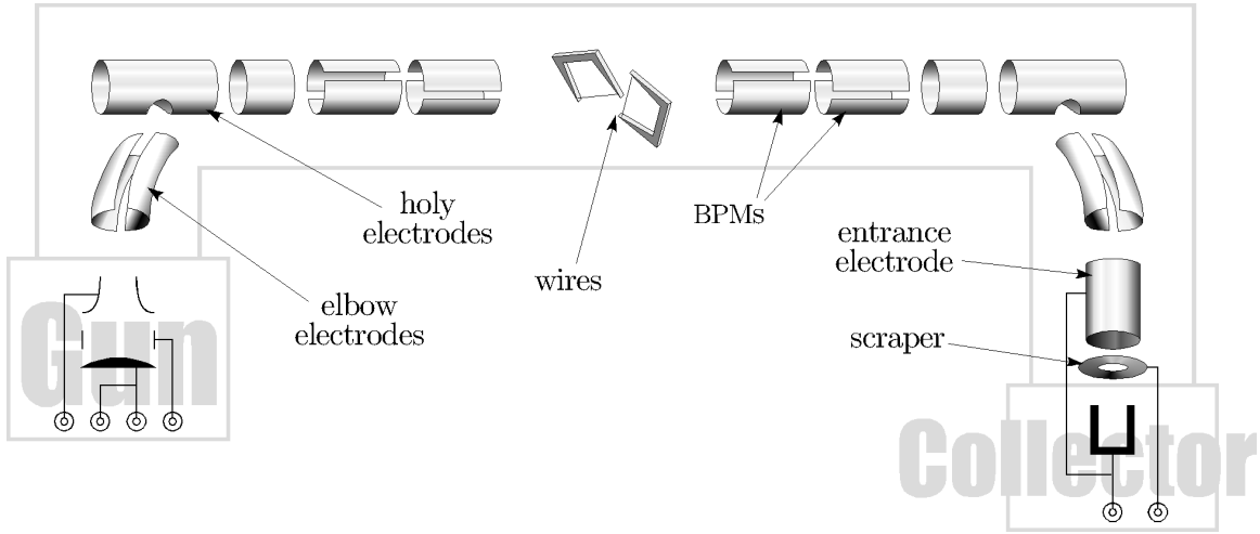
Figure 5.20. Sketch of the electrodes in the T_{EL} . While not to scale, a qualitative picture of the shape of each electrode is given.
