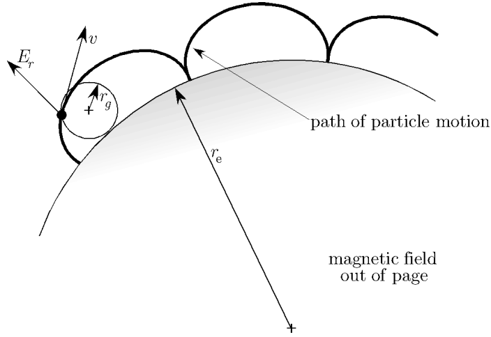
Figure 4.4. Motion of a particle in a solenoidal magnetic field and radial electric field. This motion is found to be nonrelativistic and does not affect movement along the longitudinal solenoidal field. The longitudinal motion, however, increases the relativistic mass, which in turn influences the cycloidal radius.
