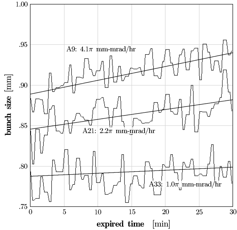
Figure 7.12. Evolution of three bunch sizes during the first thirty minutes of collisions in store #2540. A line was fitted to each of the bunches to determine their average growth rate. Antiproton bunch A33 clearly grows at a much slower pace than its siblings.
