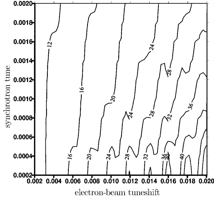
Figure 6.4. Contours of minimum magnetic field strength for a range of T EL tune-shifts and synchrotron tunes. Typical operation sets the tuneshift \Delta\nu = \sqrt{\Delta\nu_x \Delta\nu_y} at less than 0.01 and the synchrotron tune \nu_s greater than 0.0003.
