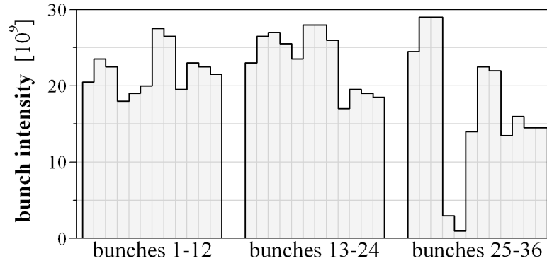
Figure 7.20. Antiproton-bunch intensities after the crazed T_{EL} interfered with the store. Bunches A28 and A29 are nearly completely eliminated, and A30 was also slightly affected.
