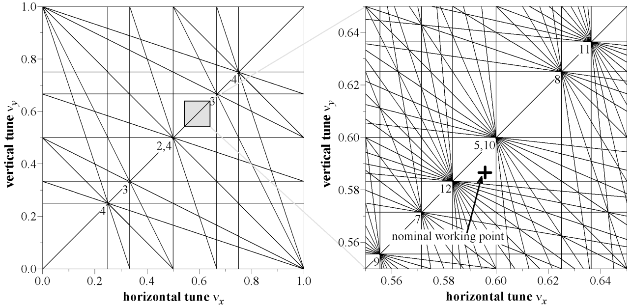
Figure 2.6. Tune plots depicting sum resonances. The left side covers the entire tune landscape and shows resonance lines through the fourth order (enumerated). The right side zooms in on a small section and includes resonances through the twelfth order.
