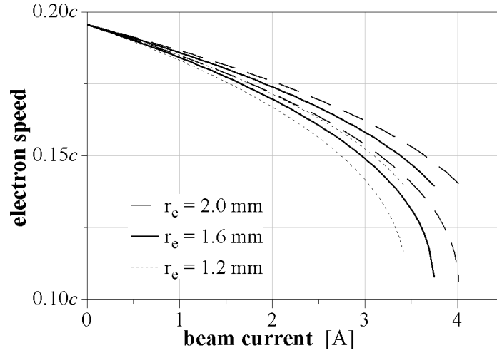
Figure 4.11. Relationship between the speed of the beam center and the total current pushed through the beam pipe, assuming V_{\text{cat}} = 10 kV. With negligible current, both the center and edge of the beam move at nearly 0.2c . As the current is increased to the maximum, the center slows to less than 0.12c .
