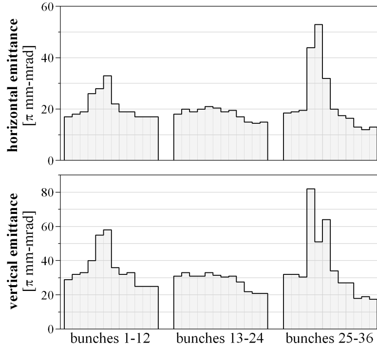
Figure 7.21. Horizontal and vertical emittance measurements after the current fluctuations nearly obliterated bunches A28 and A29. All of the touched bunches show significantly increased emittances.
