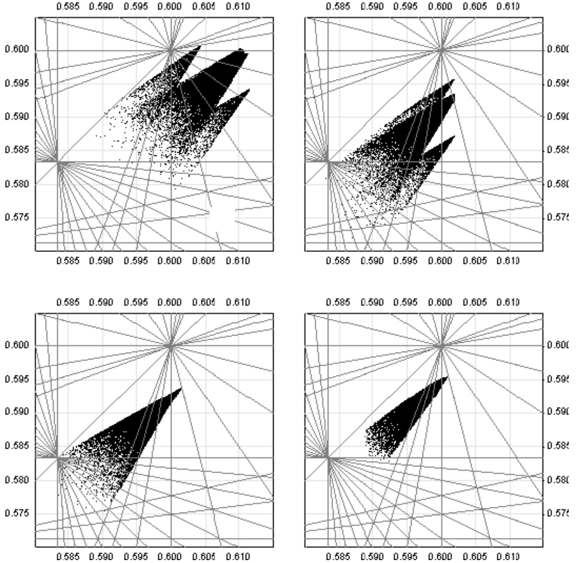
Figure 3.1. Examples of schemes for beam-beam compensation. The upper-left situation shows the original unperturbed antiproton footprint. The upper-right diagram shows the footprint if linear compensation is applied to each of the bunches, but the horizontal and vertical shifts are not independently controlled. The lower-left case allows independent control of horizontal and vertical tunes, so that all 36 bunches lie on top of each other. In the lower-right situation, nonlinear compensation is added to the linear, creating a dramatically small footprint. These simulations of the Tevatron used tracking codes and the insertion of one or two T F Ls at different places around the ring.
