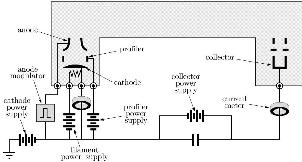
Figure 5.26. Oversimplified schematic of the TFL circuitry. In this picture, the power supplies are located close to the TFL, and the anode, filament, and profiler voltages are referenced to stable cathode voltage.
