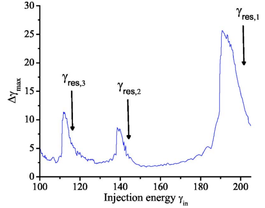
FIG. 6. (Color online) Maximum energy gain (in units of mc^2 ) of particles injected in a IFEL accelerator at different energies. The vertical arrows indicate the higher harmonic IFEL resonant energies \gamma_{r,n} with n=1,2,3 .
