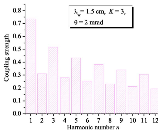
FIG. 7. (Color online) Coupling strength K J_n(K) vs harmonic number n .
