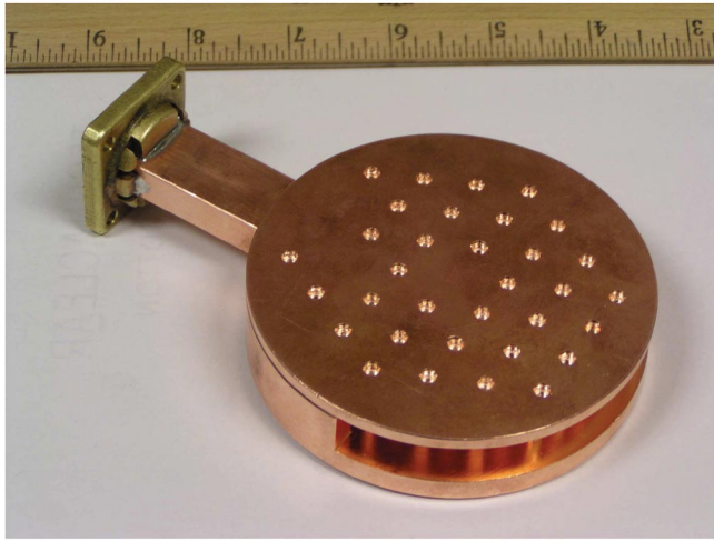
FIG. 7. (Color) Brazen PBG resonator.
