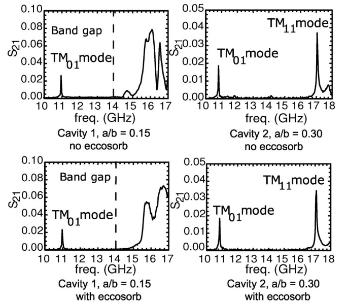
FIG. 6. Cold test measurements of the transmission coefficient S_{21} for the brass resonators cavity 1 and cavity 2.
