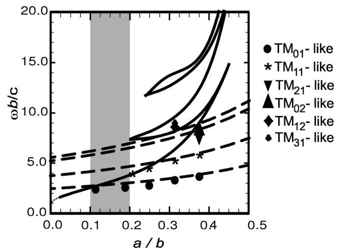
FIG. 2. The eigenfrequencies of the TM modes in PBG cavity formed by a single removed rod from the triangular lattice. The eigenfrequencies are plotted with dots for different ratios of a/b . Black solid lines show the band gap boundaries. Dashed lines represent the frequencies of modes of a pillbox cavity with the radius R = b - a . For the values of a/b inside the shaded region the PBG resonator only confines a single, TM 01 -like mode.
