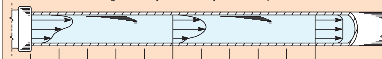
Figure 5: Non-symmetrical and symmetrical flow profiles
