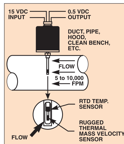
Figure 1: Insertion style mass flow sensor utilizes RTD sensor to measure the flow rate
