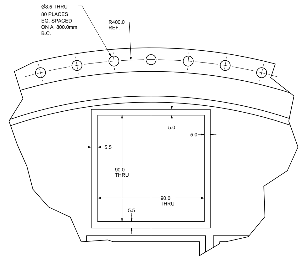
DETAIL T SCALE 1 : 1
