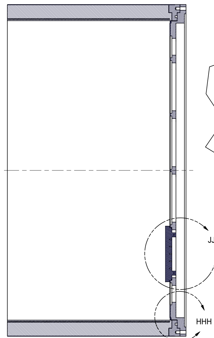
SECTION GGG-GGG SCALE 3/8
