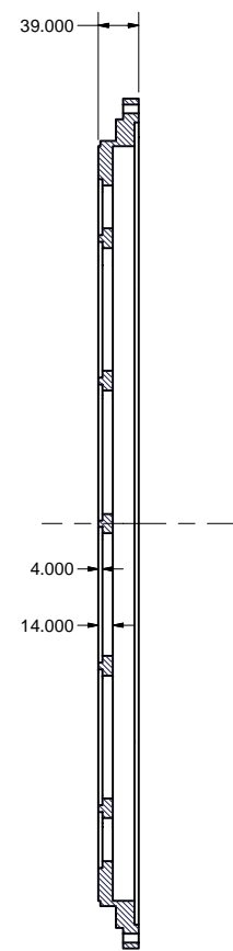
SECTION JJ-JJ SCALE 1 / 4
