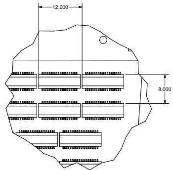
DETAIL PPP SCALE 3:1
