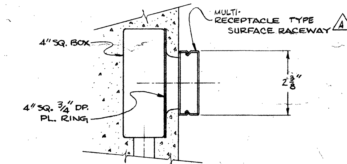
SHOP & EQUIPMENT AREA SURFACE RACEWAY DETAIL 1 SCALE: 1/2" = 1'-0"
