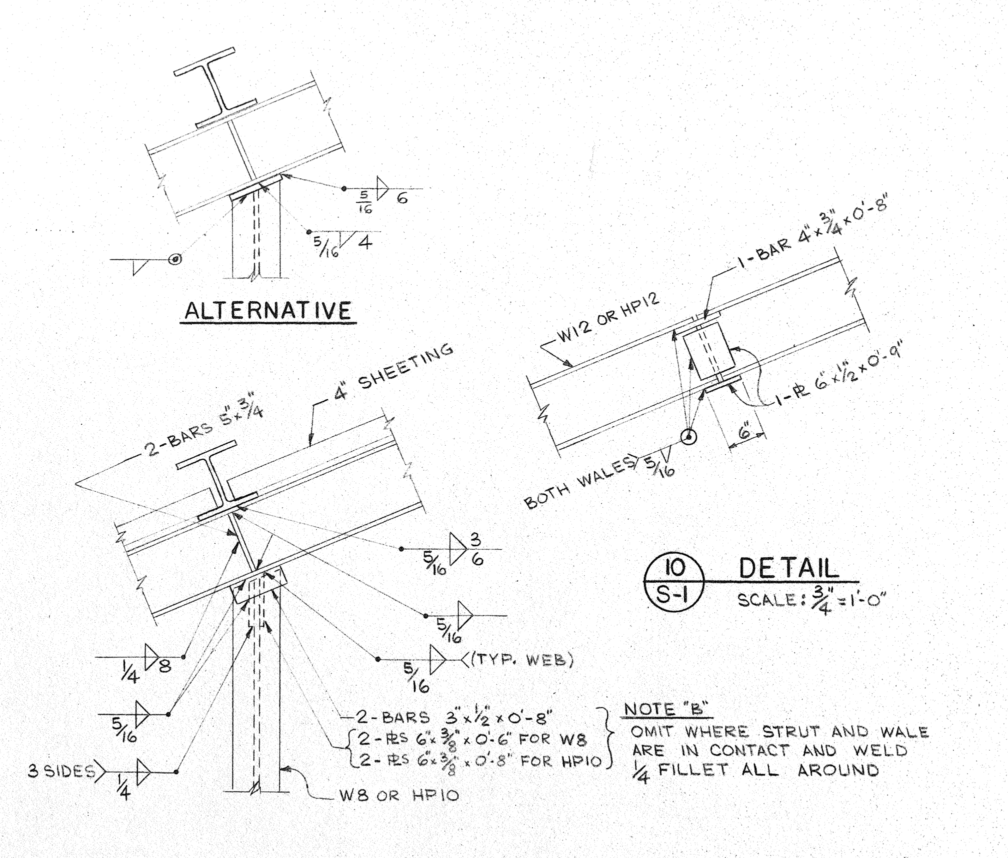
8 DETAIL SCALE: 3/4\"/>
