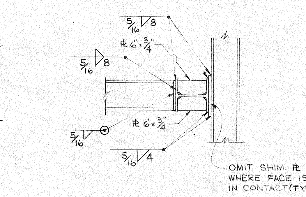
4 DETAIL SCALE: 3/4\"/>
