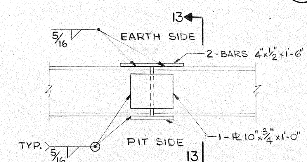
3 DETAIL SCALE: 3/4\"/>
