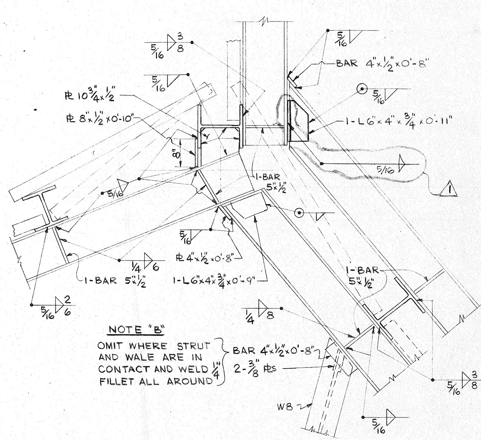
2 DETAIL SCALE: 3/4\"/>
