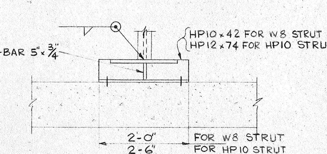
9 DETAIL SCALE: 3/4\"/>
