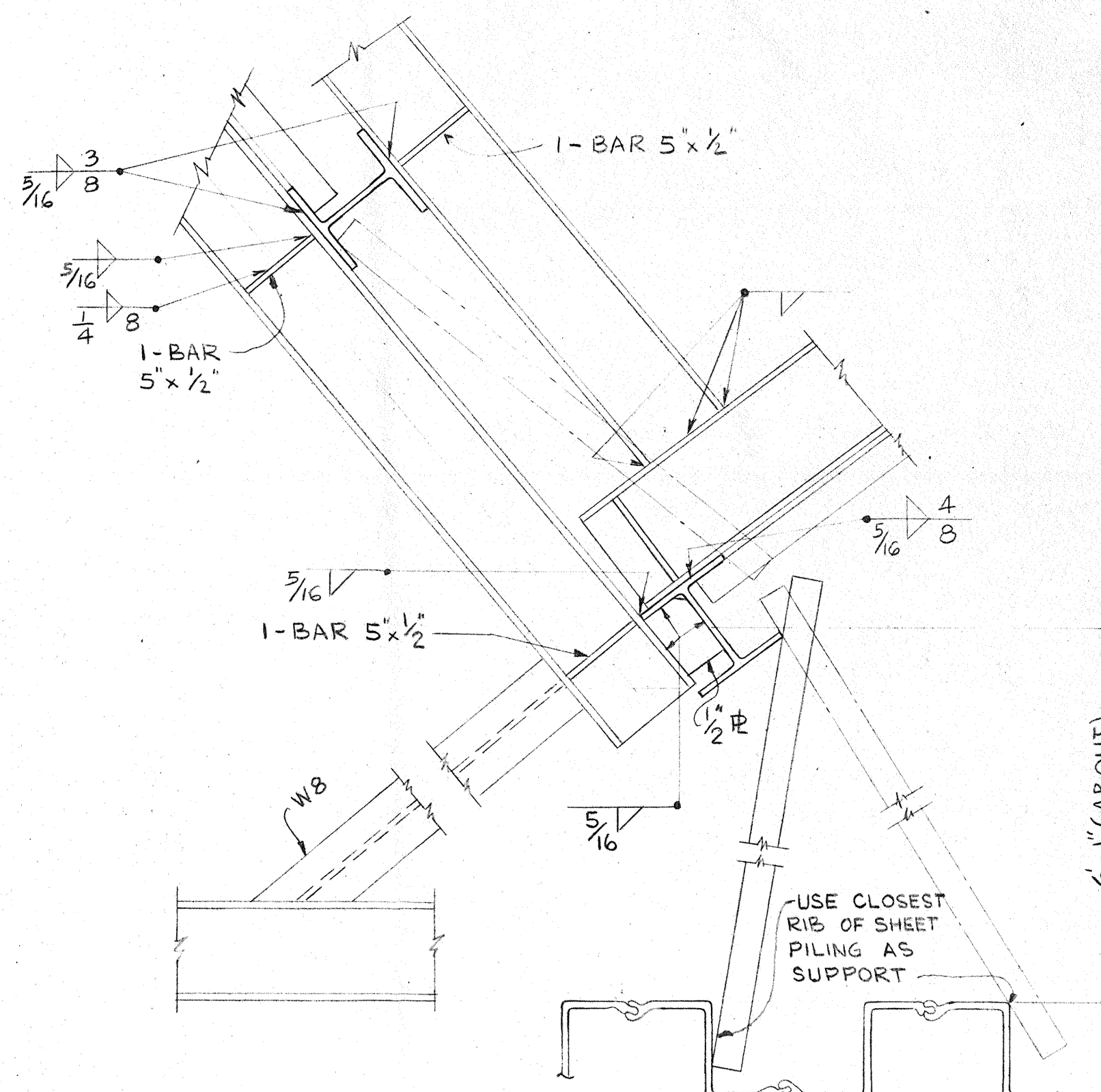
5 DETAIL SCALE: 3/4\"/>
