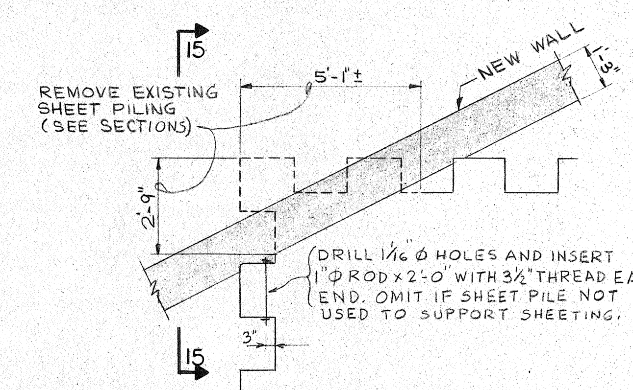
11 DETAIL SCALE: 3/8\"/>
