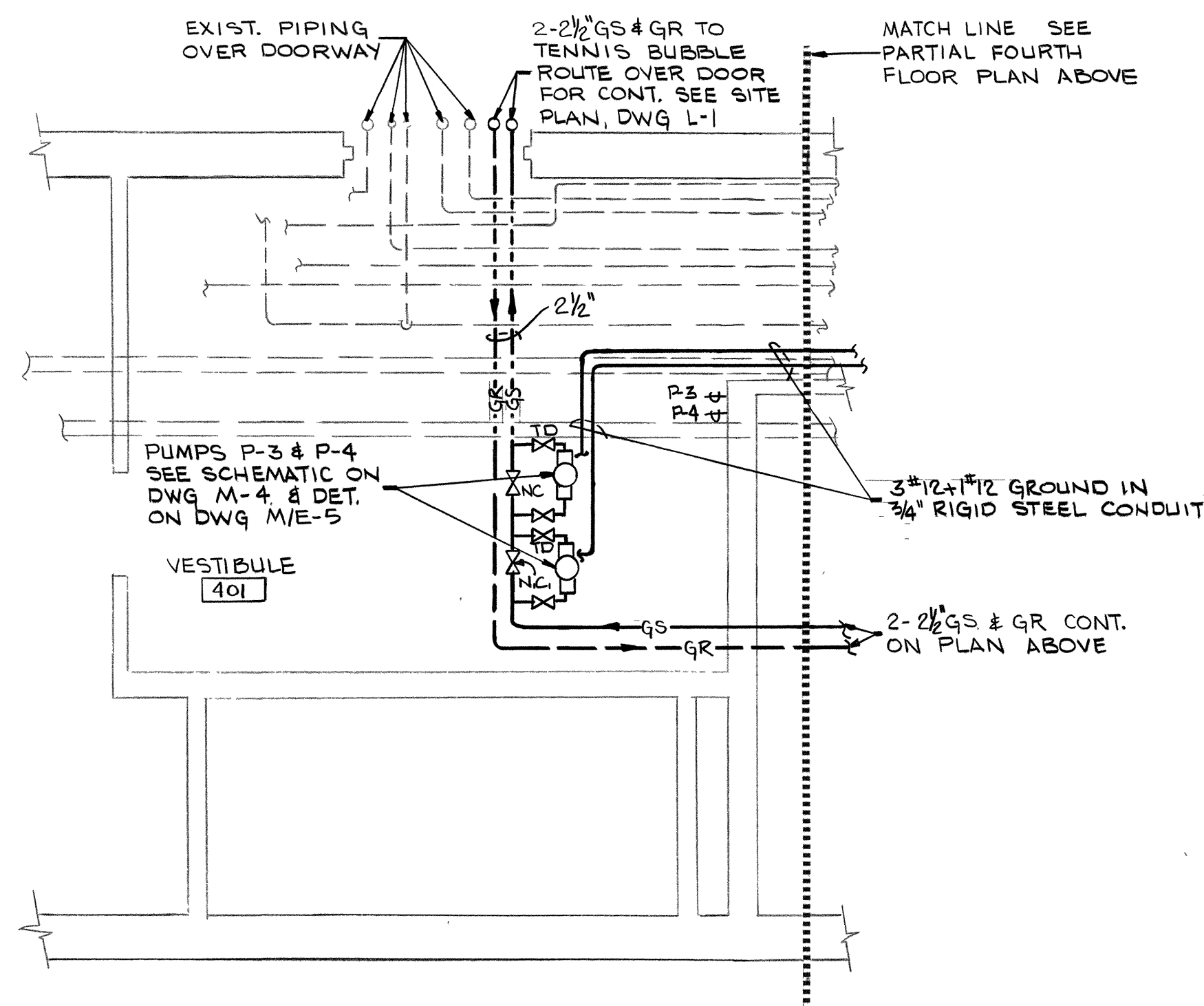
PARTIAL FOURTH FLOOR PLAN SCALE 1/4"=1'-0"
