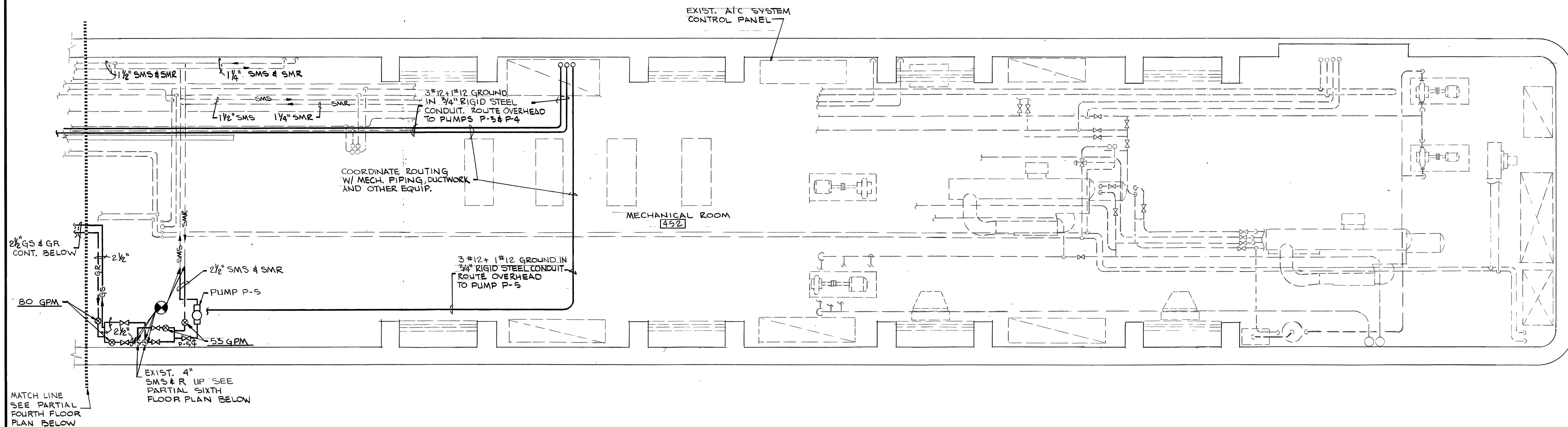
PARTIAL FOURTH FLOOR PLAN SCALE 1/4"=1'-0"
