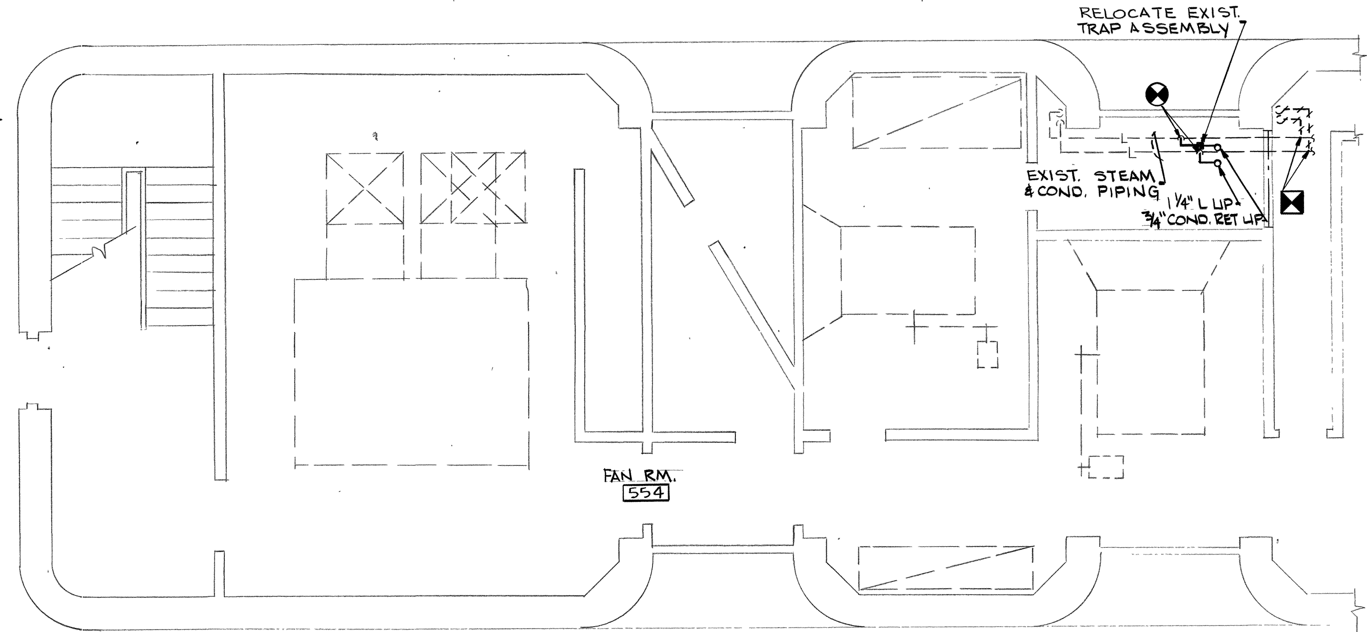
PARTIAL FIFTH FLOOR PLAN SCALE 1/4"=1'-0"
