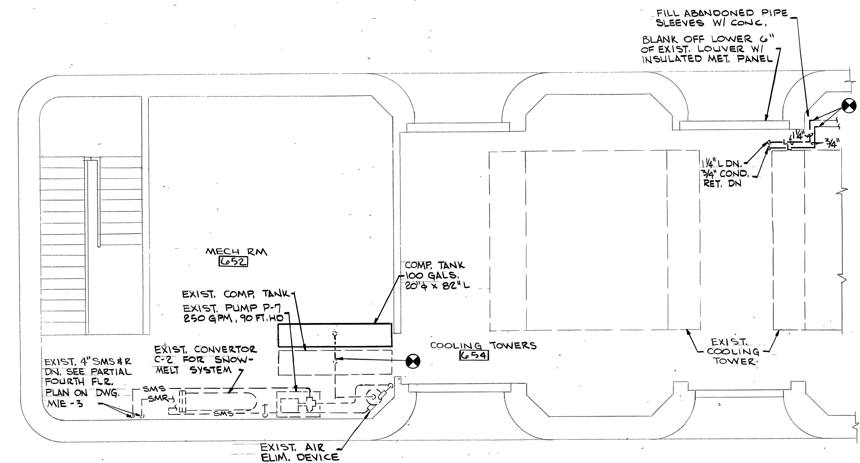
PARTIAL SIXTH FLOOR PLAN SCALE 1/4"=1'-0"
