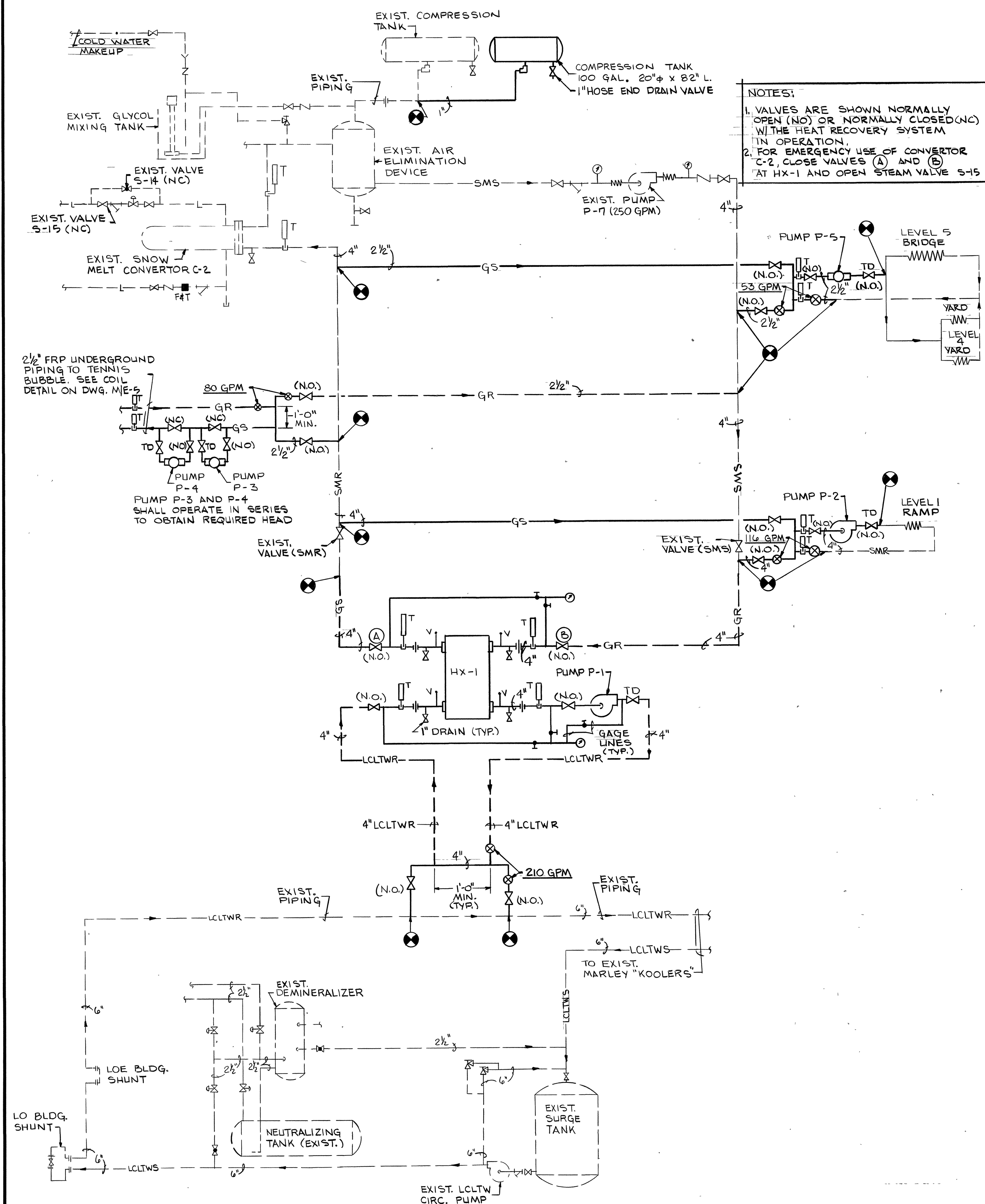
LCLTW HEAT RECOVERY PIPING SCHEMATIC NO SCALE
