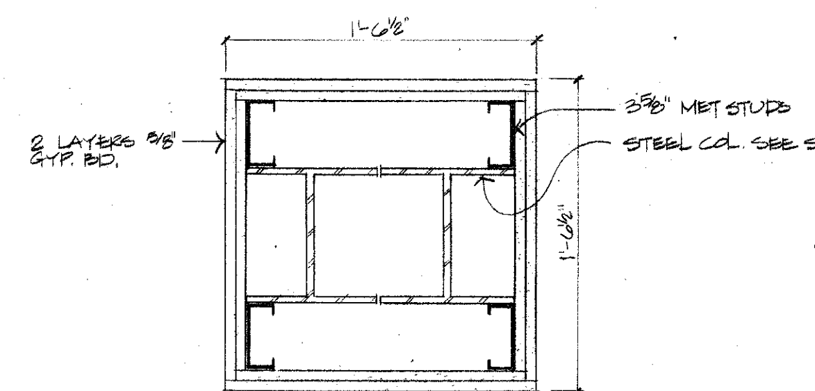
4 GYP BD SHEATHING AT STEEL COLUMNS A3 1/2" = 1'-0"
