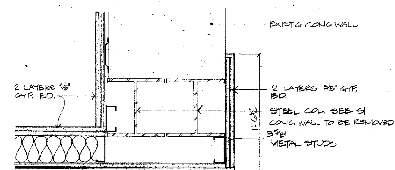
3 GYP BD SHEATHING AT STEEL COLUMNS A3 1/2" = 1'-0"
