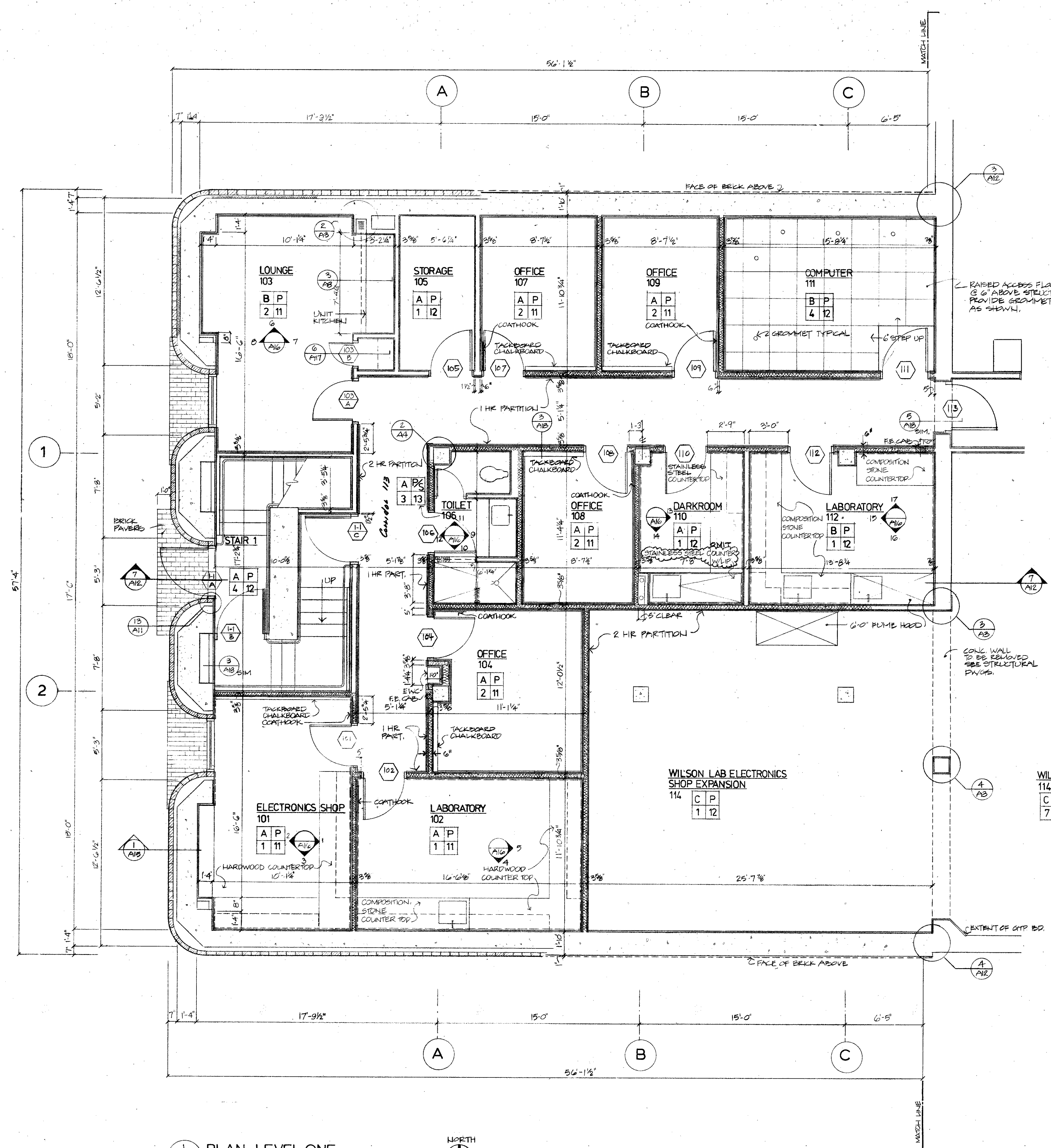
1 PLAN-LEVEL ONE A3 1/4" = 1'-0"
