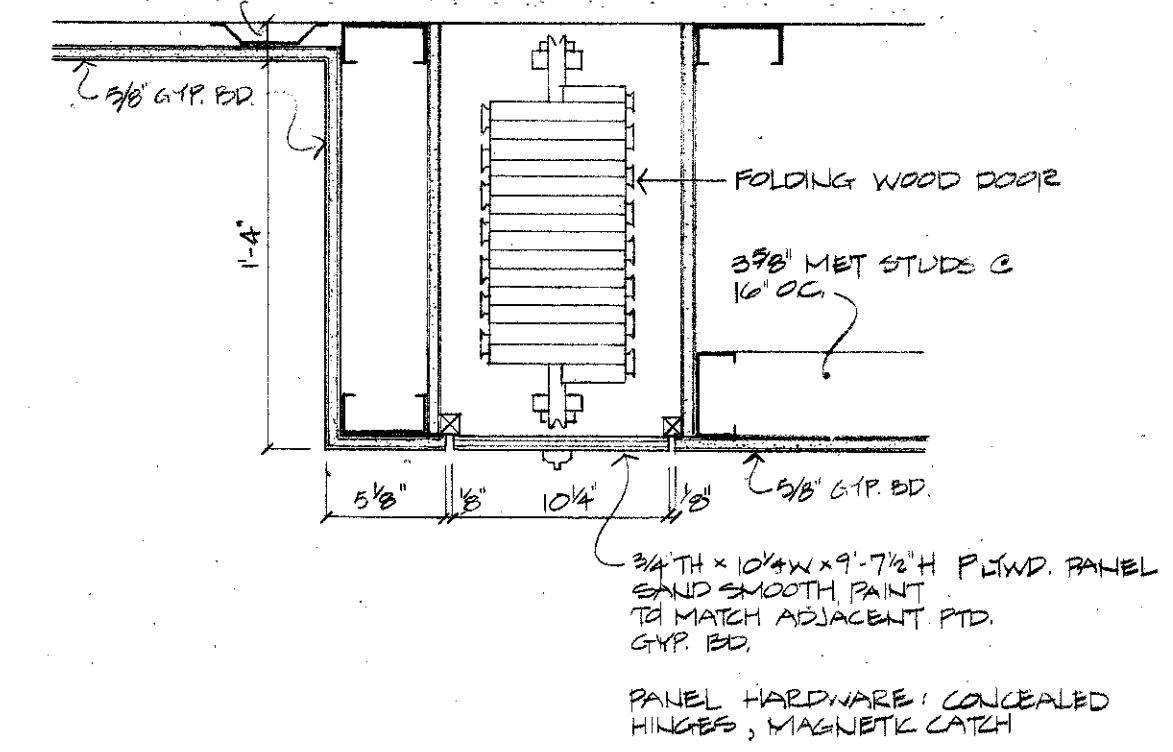
2 FOLDING WOOD DOOR POCKET A3 1/2" = 1'-0"
