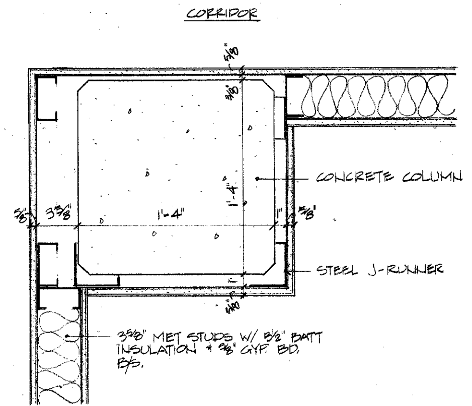
2 FURRING AT COLUMN A4 1/2" = 1'-0"
