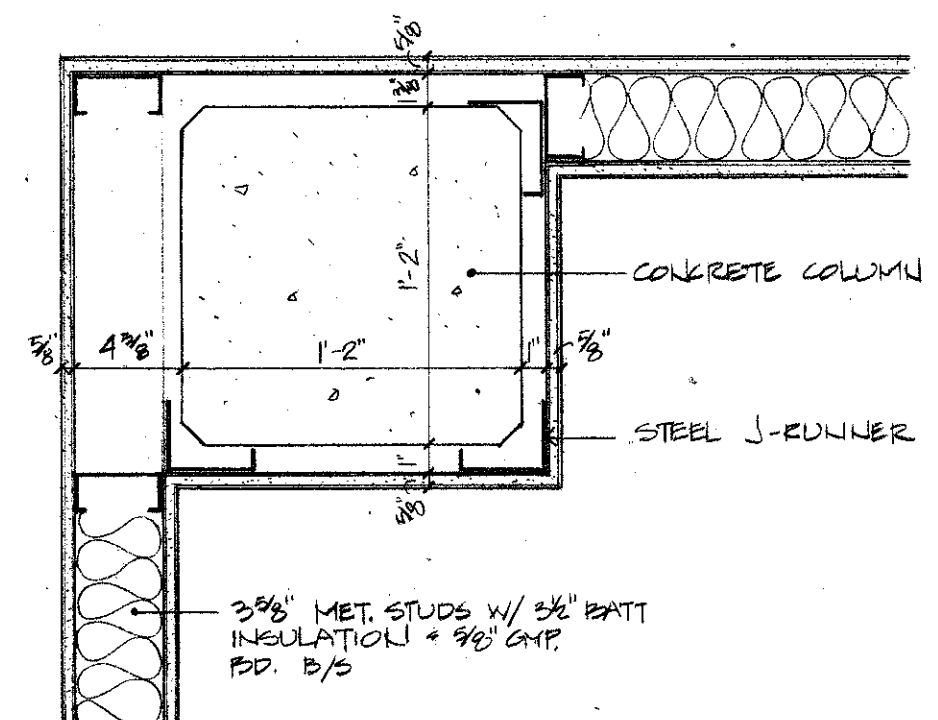
3 FURRING AT COLUMN A4 1/2" = 1'-0"
