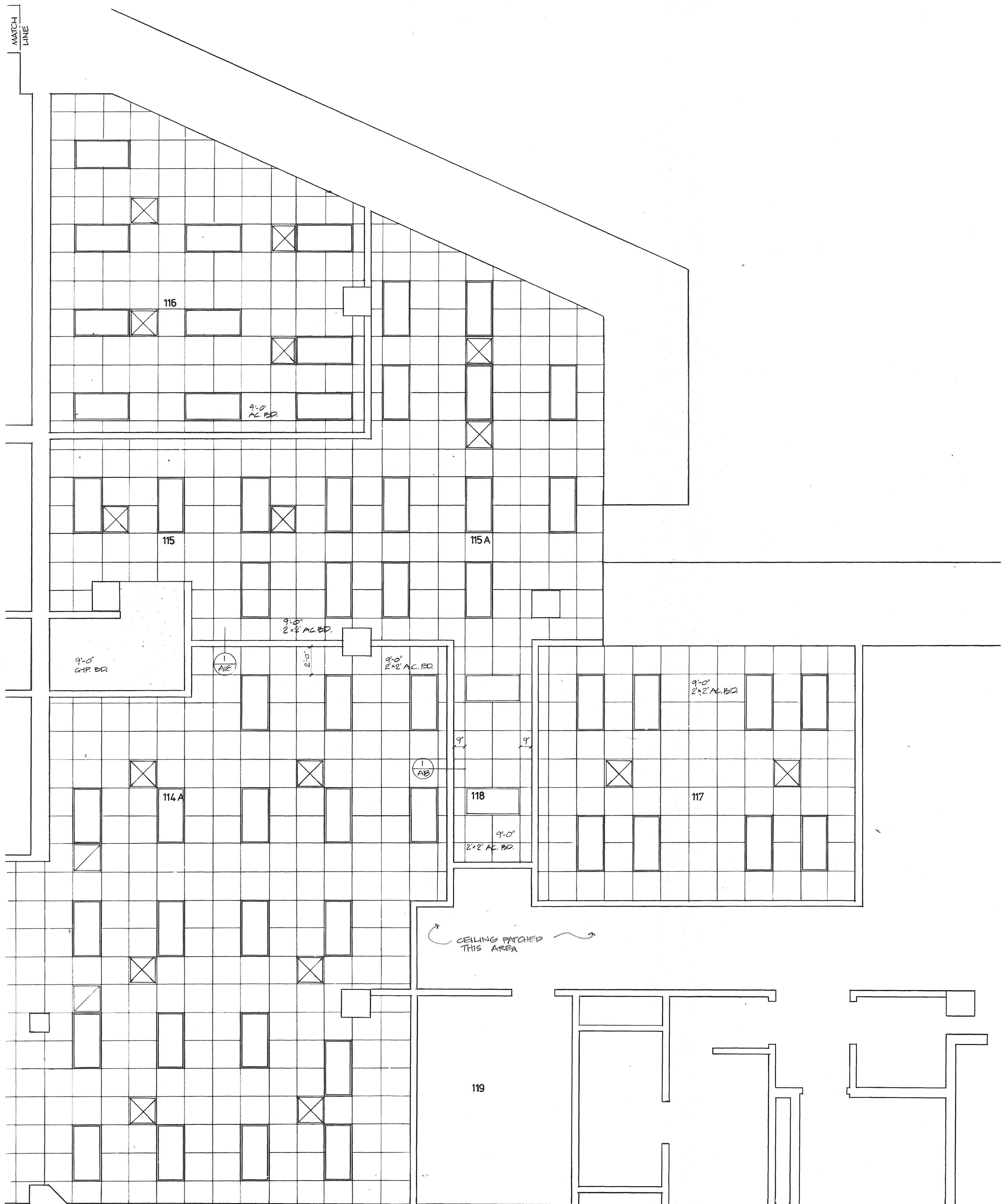
1 LEVEL ONE, EXISTING- REFLECTED CEILING PLAN 1/4" = 1'-0"
