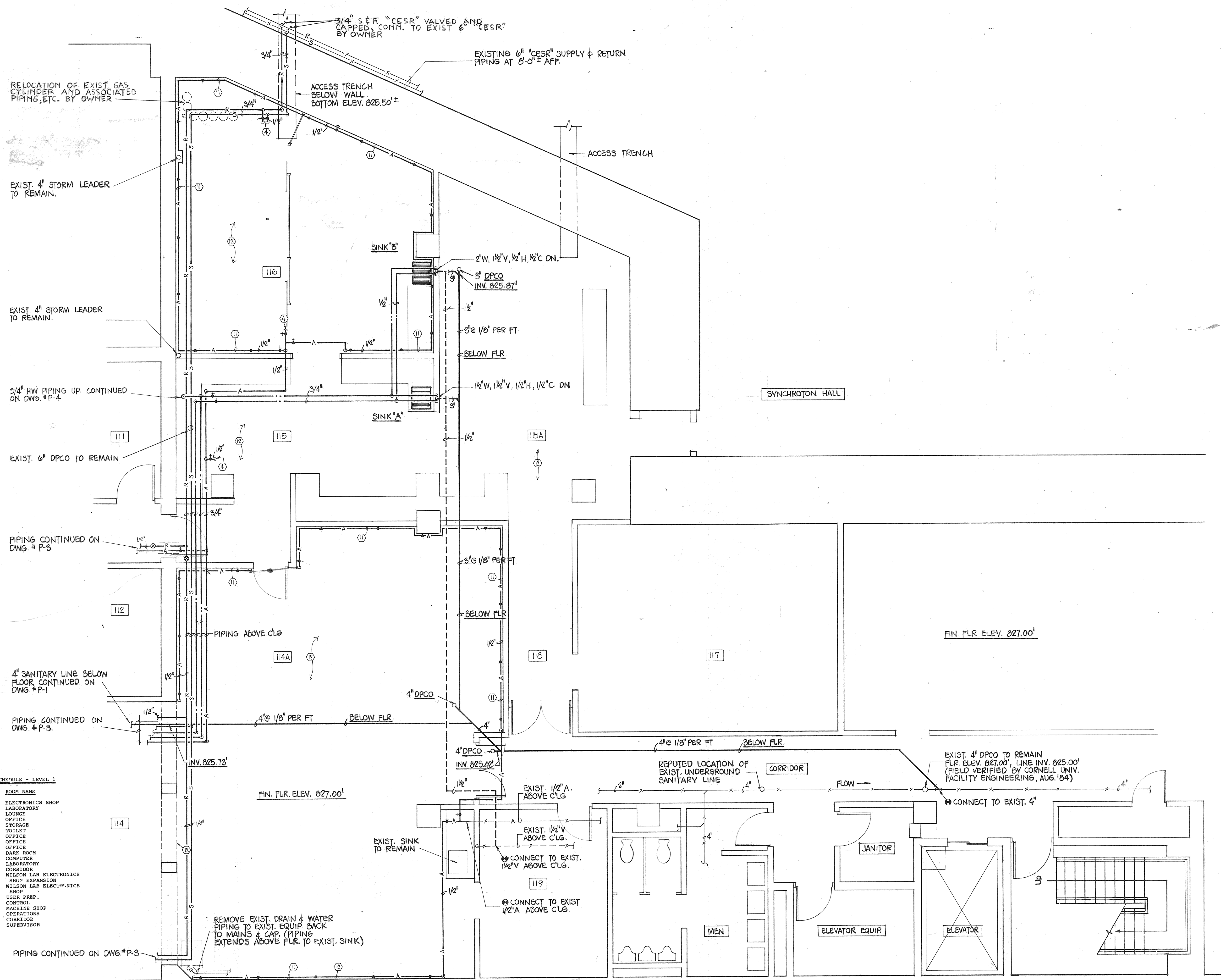
LEVEL ONE - EXISTING - PLUMBING
