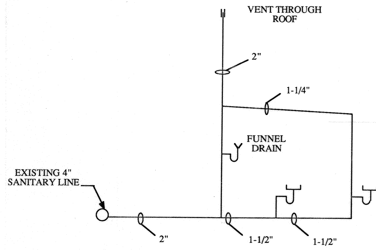
DRAIN RISER SCHEMATIC NOT TO SCALE
