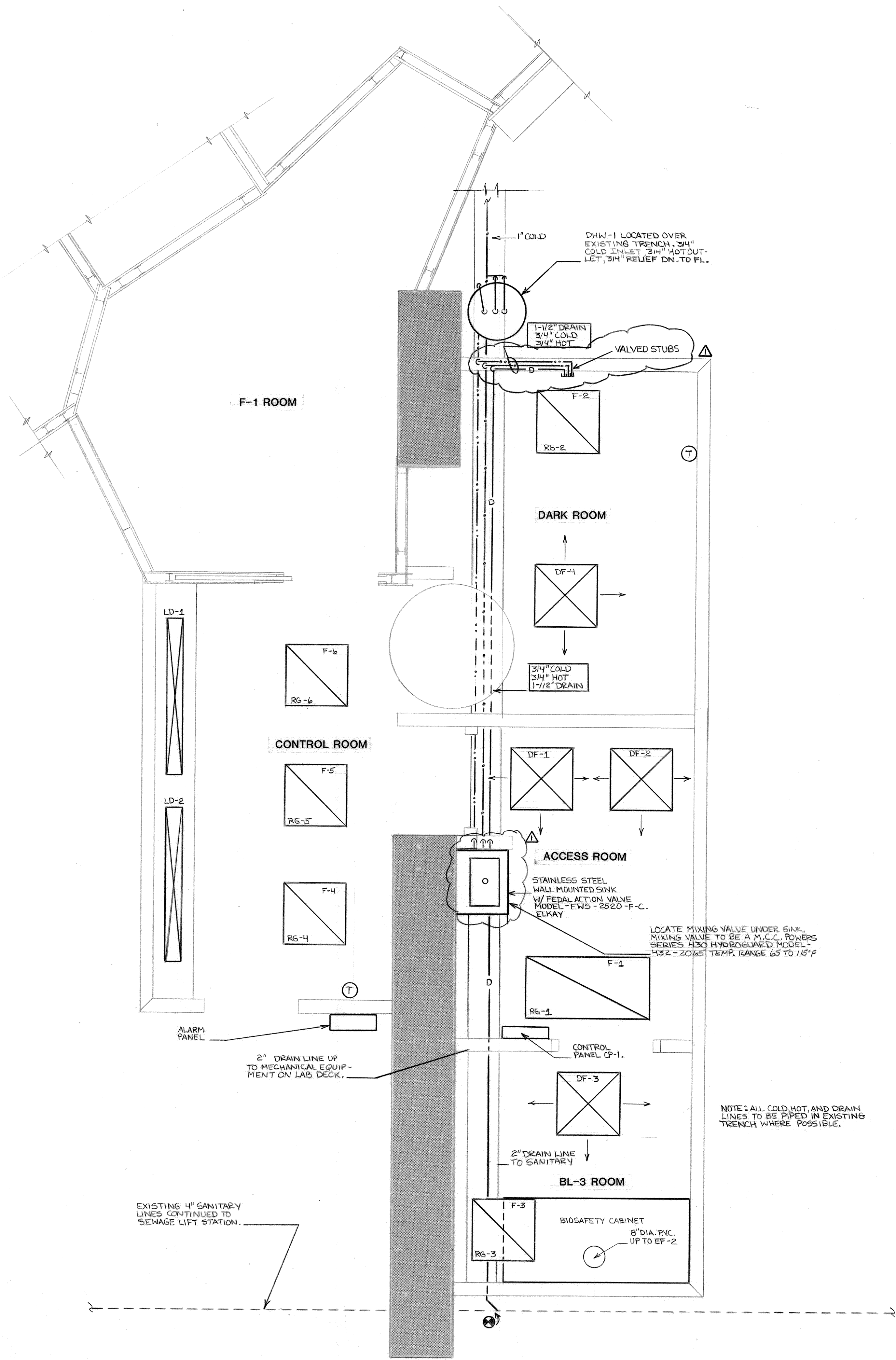
LAB PLAN SCALE 1/2" : 1'-0"
