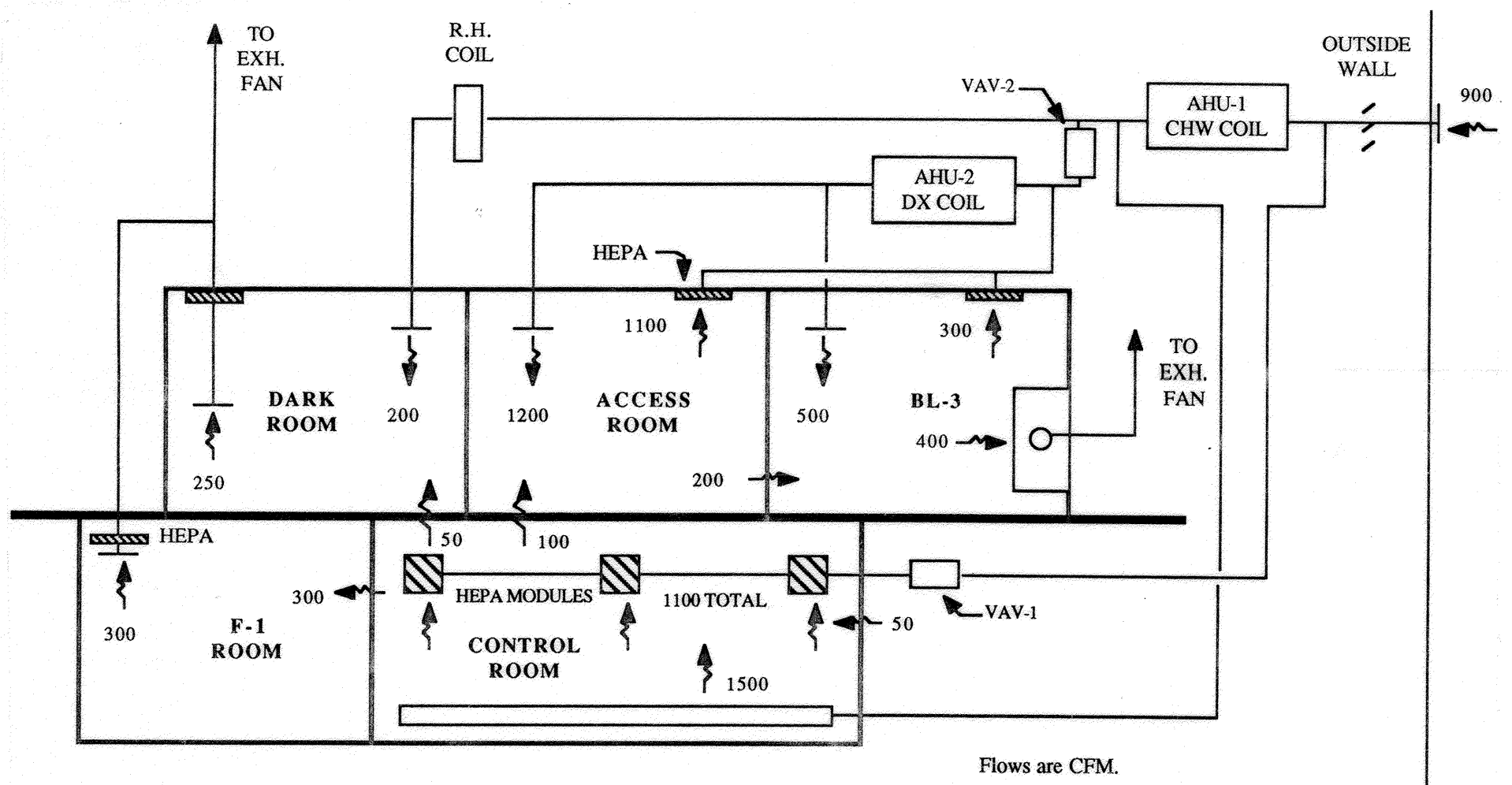
MECHANICAL SYSTEM SCHEMATIC NOT TO SCALE
